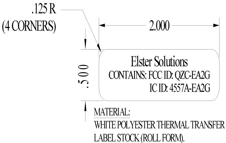
Figure 2: External FCC / IC Label Drawing
