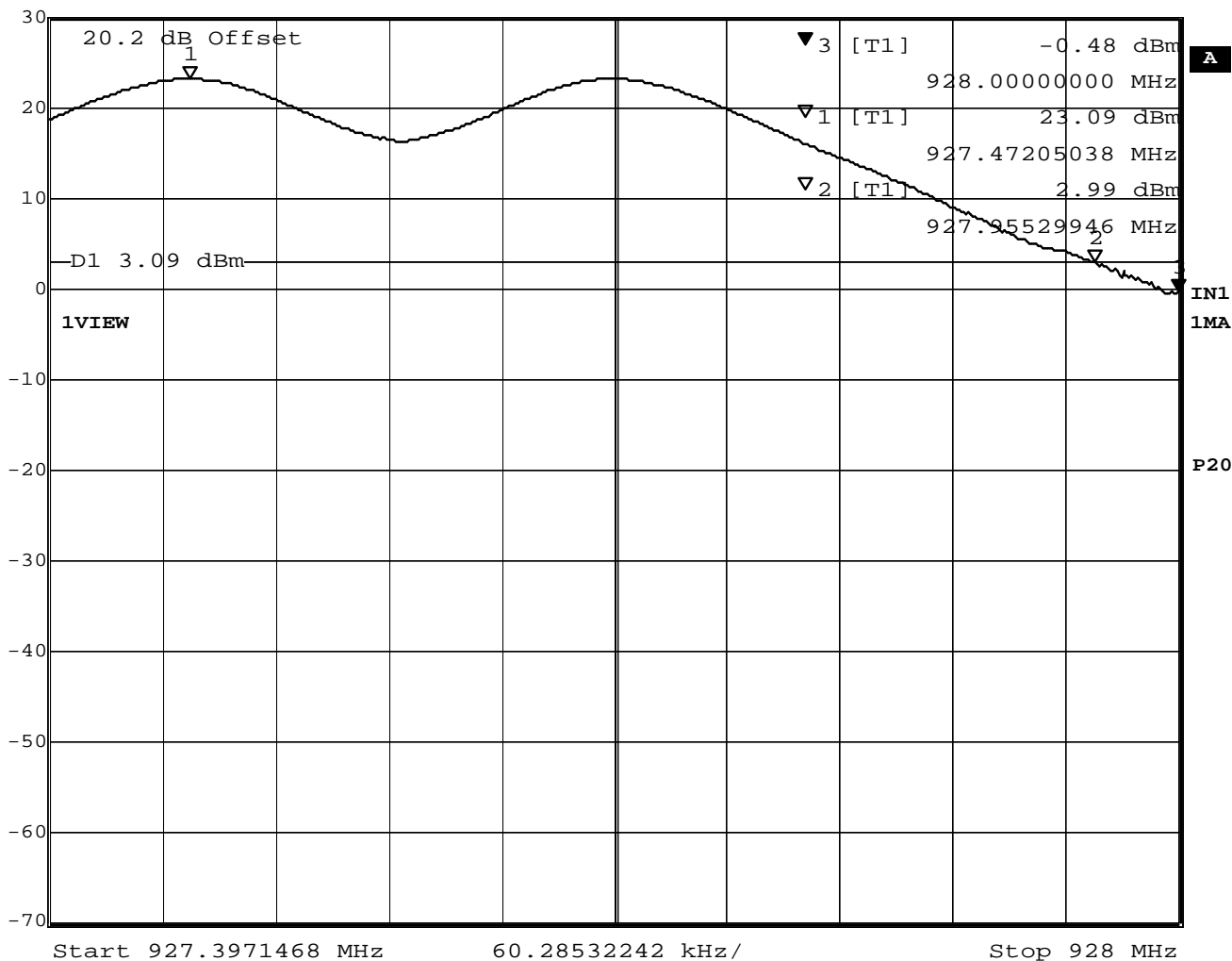
Figure 6: Upper Band Edge Measurement
