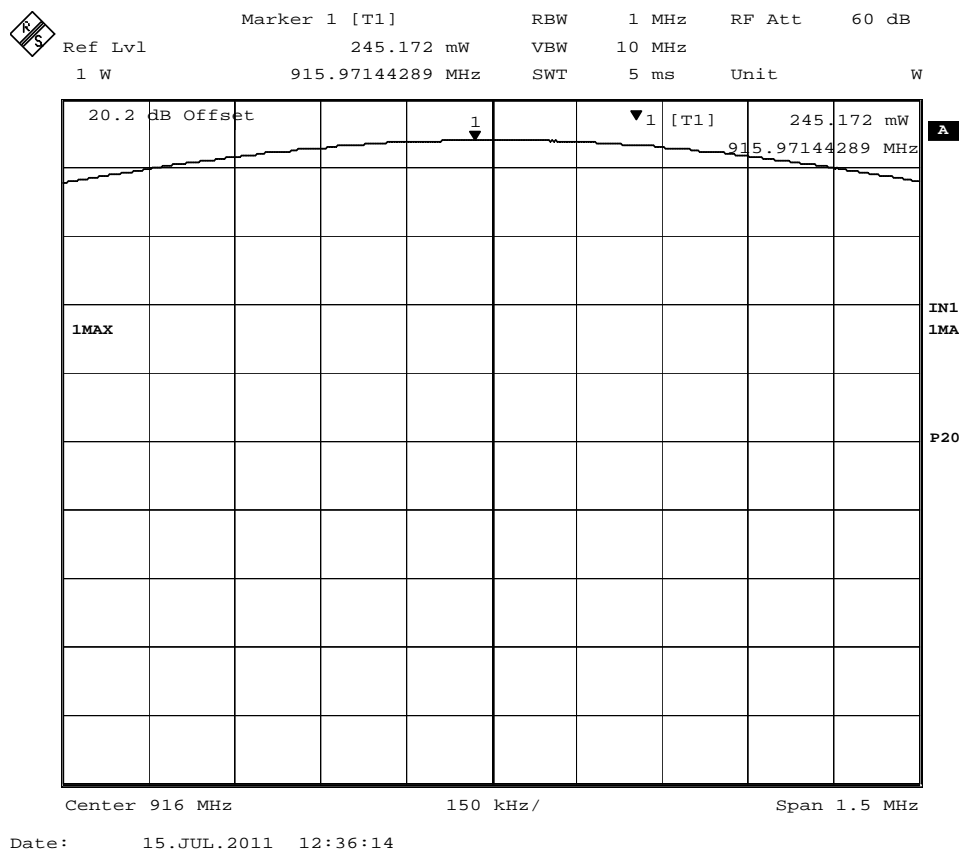
Figure 7: CH 34 (916.0 MHz) Peak Output Power - Worst Case Shown. Plots of other channels are on file at TUV Rheinland.
