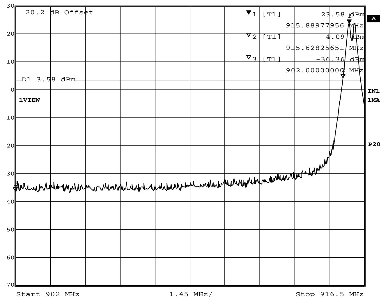
Figure 5: Lower Band Edge Measurement
