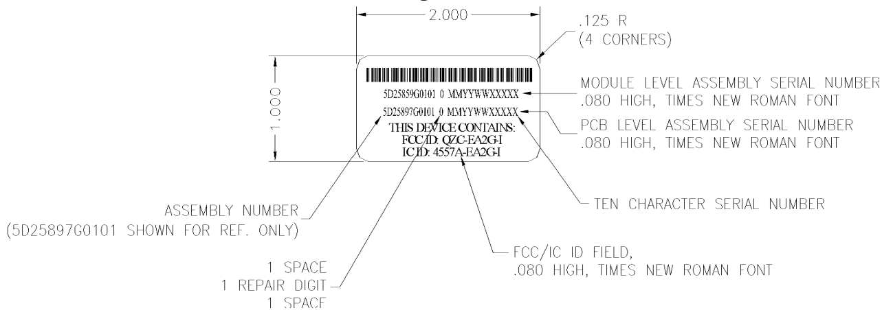
Figure 2: External FCC Label Drawing
