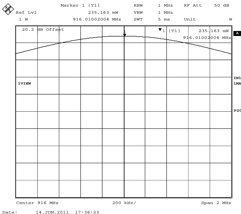
Figure 7: CH 34 (916.0 MHz) Peak Output Power - Worst Case Shown.
