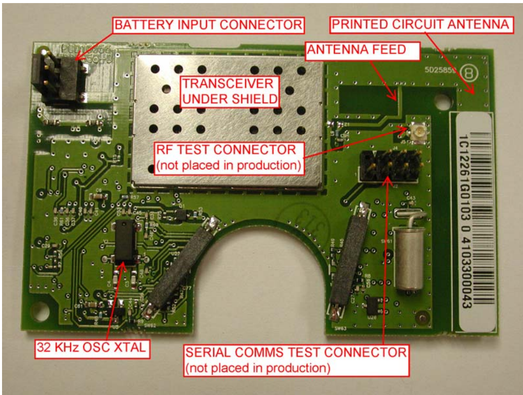
Figure 1: PCB Assembly Top View
