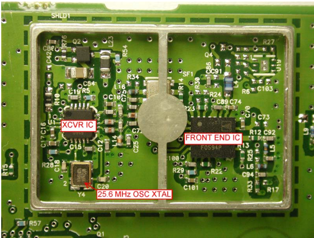
Figure 3: Transceiver Circuitry under Shield
