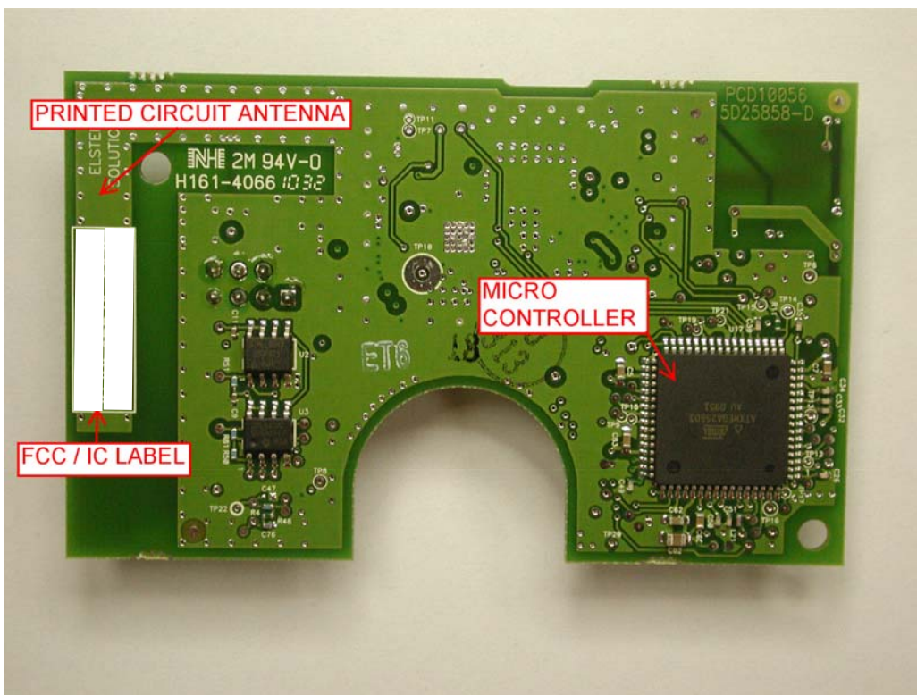
Figure 2: PCB Assembly Bottom View
