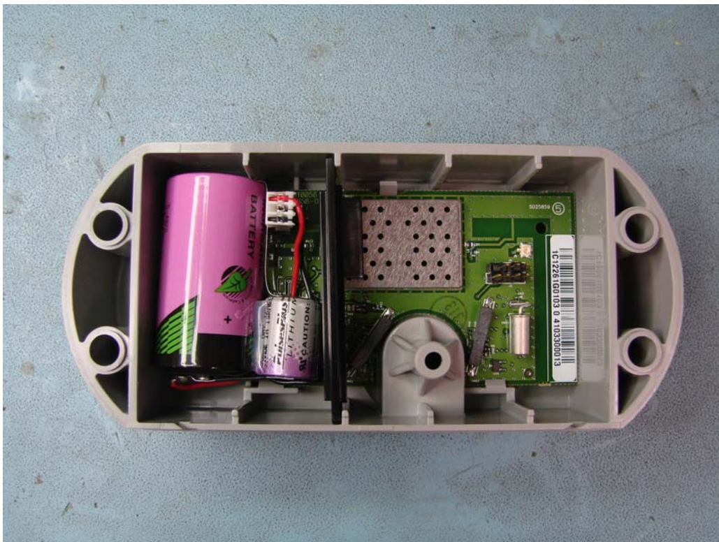
Figure 4: Assembled module prior to Potting
