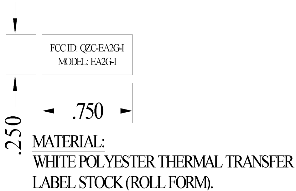
Figure 4: Internal FCC Label Drawing
