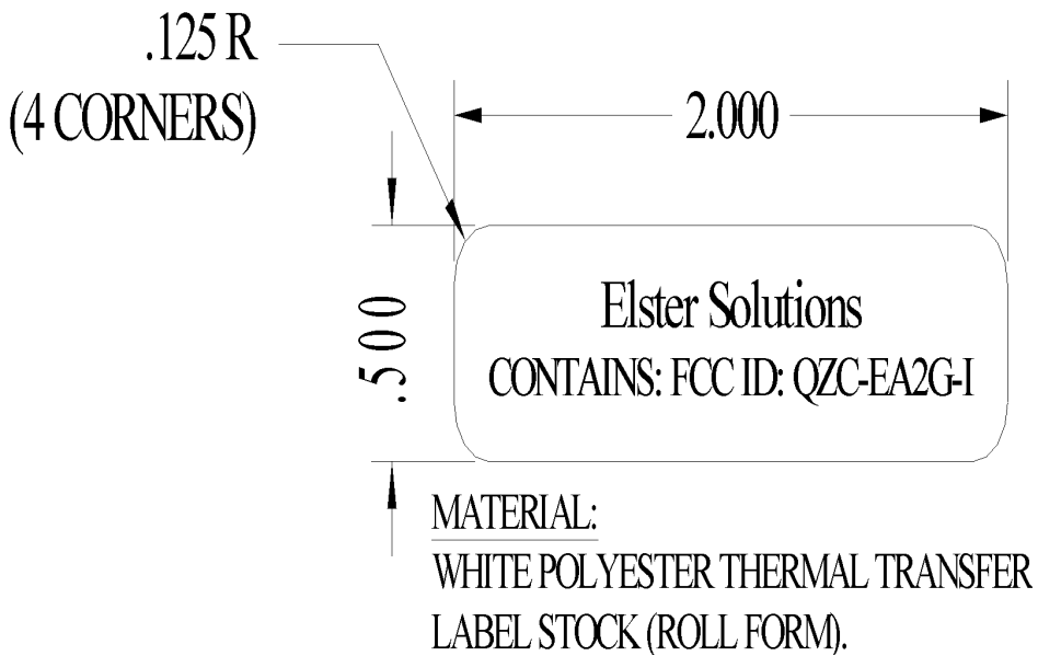
Figure 2: External FCC Label Drawing
