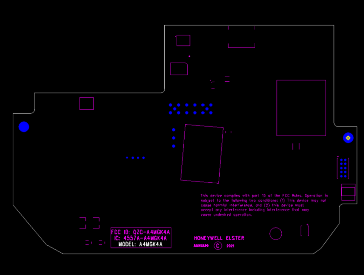
Label location on A4MGK4A PCBA
