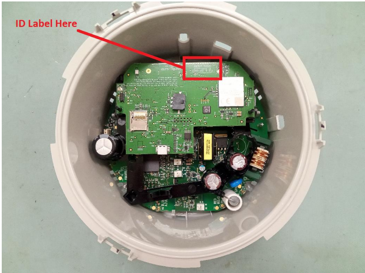
Label location as installed in A4 meter host
