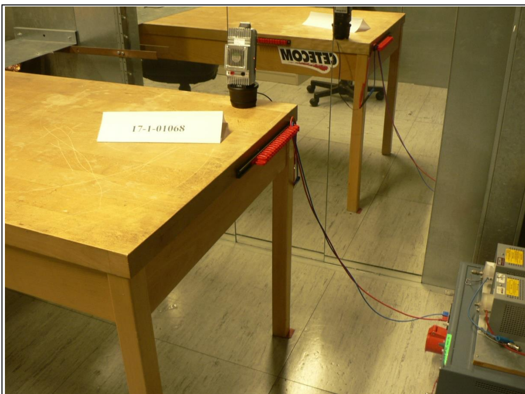
Photograph 2: Radiated measurements, EMI-on DC-mains, test set-up 5
