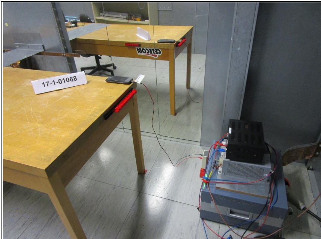
Photograph 1: Conducted measurements, EMI-on DC-mains, test set-up 2
