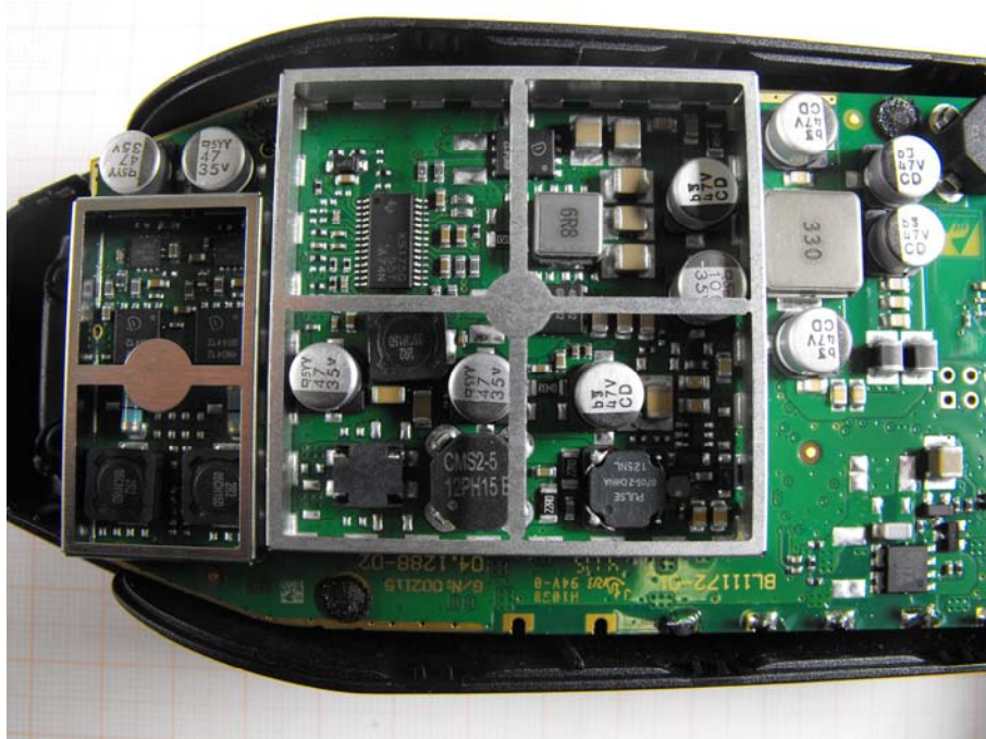
Photo 2: Main board, shielding removed
