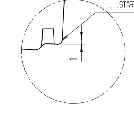
Detail F Start-Messpunkt Kontrollmess ... START MEASURING POINT
