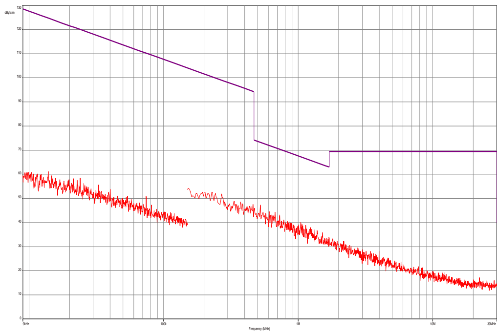
Plot 2: 9 kHz to 30 MHz, RX/Idle mode
