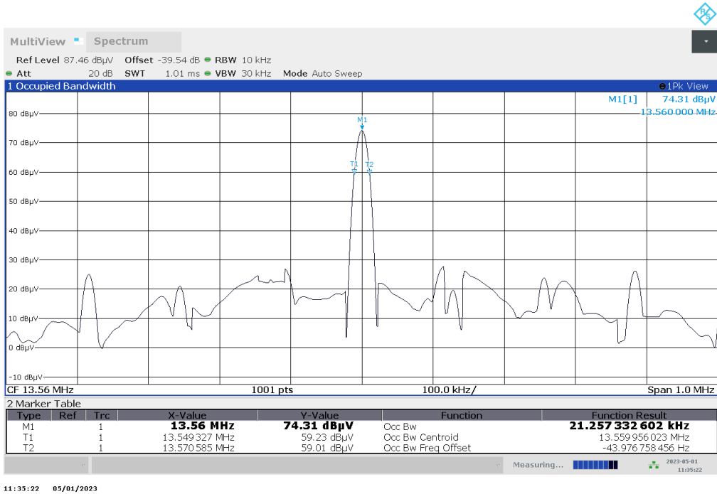
Plot no. 15: Frequency tolerance @ +80 °C, EUT A, Vmax
