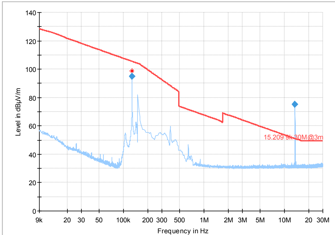
Plot no. 4: Radiated emissions 9 kHz – 30 MHz, EUT staying
