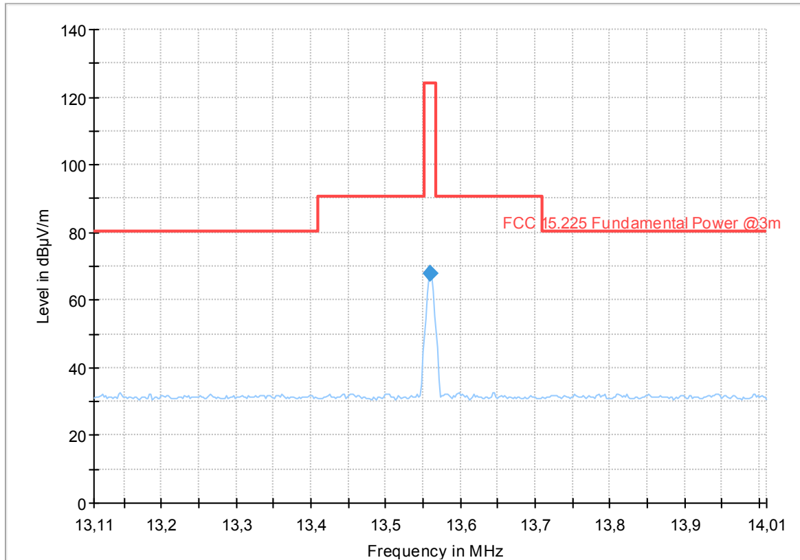
Plot no. 1: Transmitter Spectrum Mask (TSM), lying
