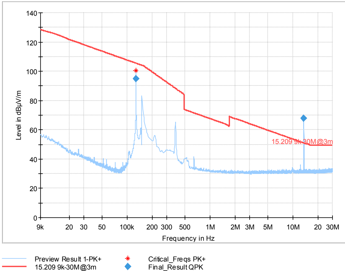
Plot no. 3: Radiated emissions 9 kHz – 30 MHz, EUT lying
