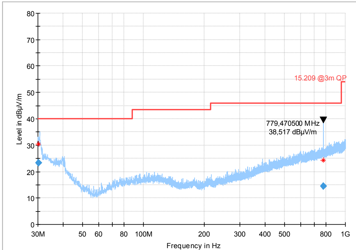
Plot no. 5: Radiated emissions 30 MHz – 1 GHz, hor./vert. polarization, EUT lying
