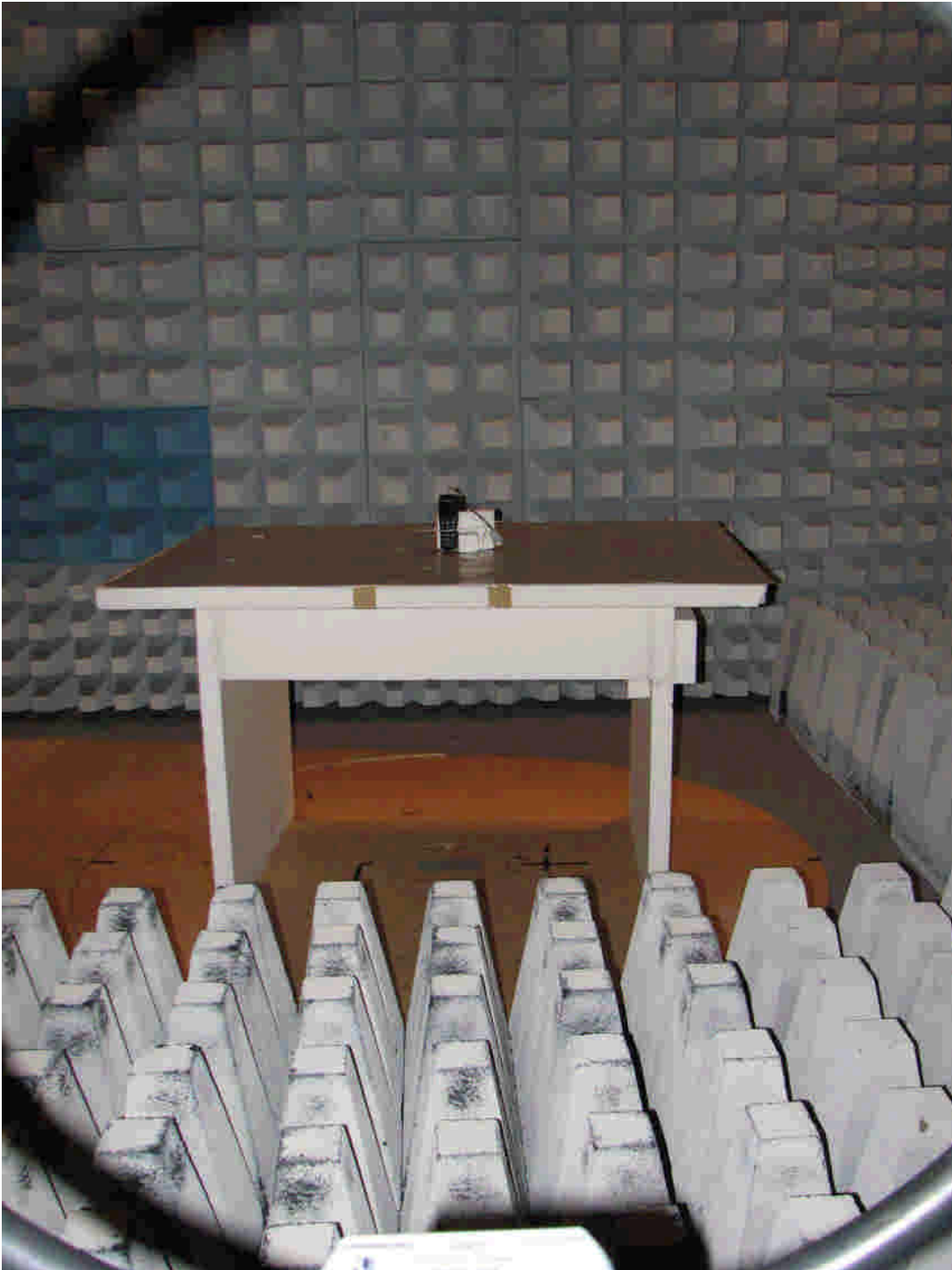
72337_11.jpg EUT, test set-up fully anechoic chamber
