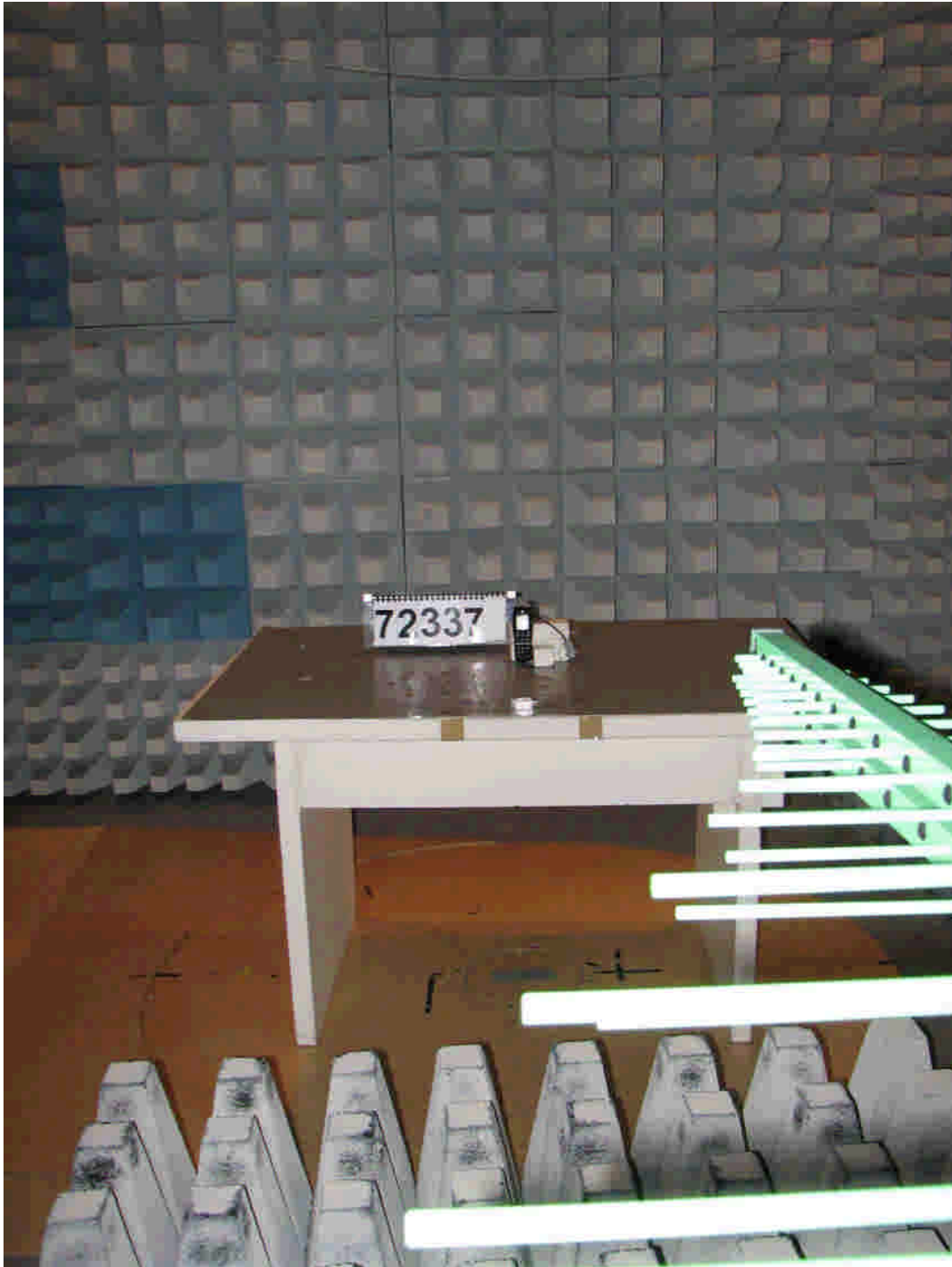
72337_12.jpg EUT, test set-up fully anechoic chamber
