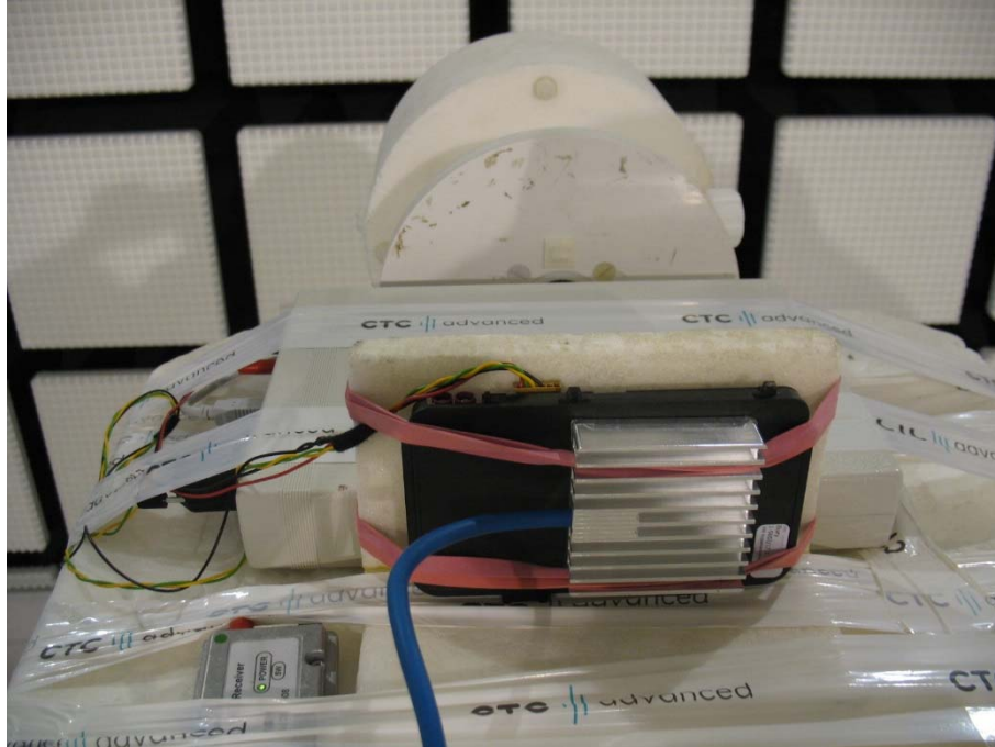
Photo 9: WPC measurements
