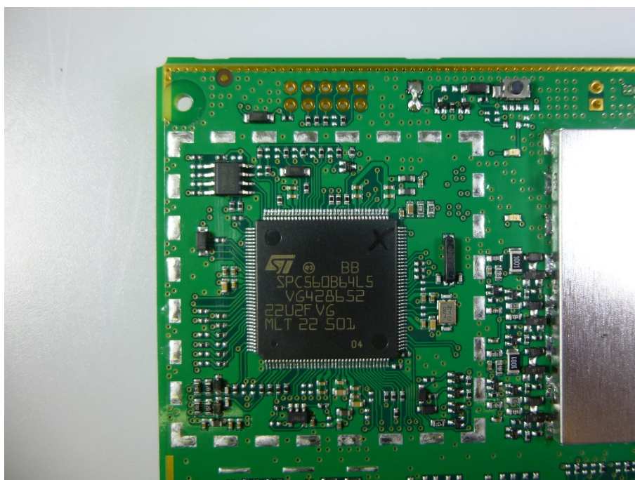
Photo 4: PCB
