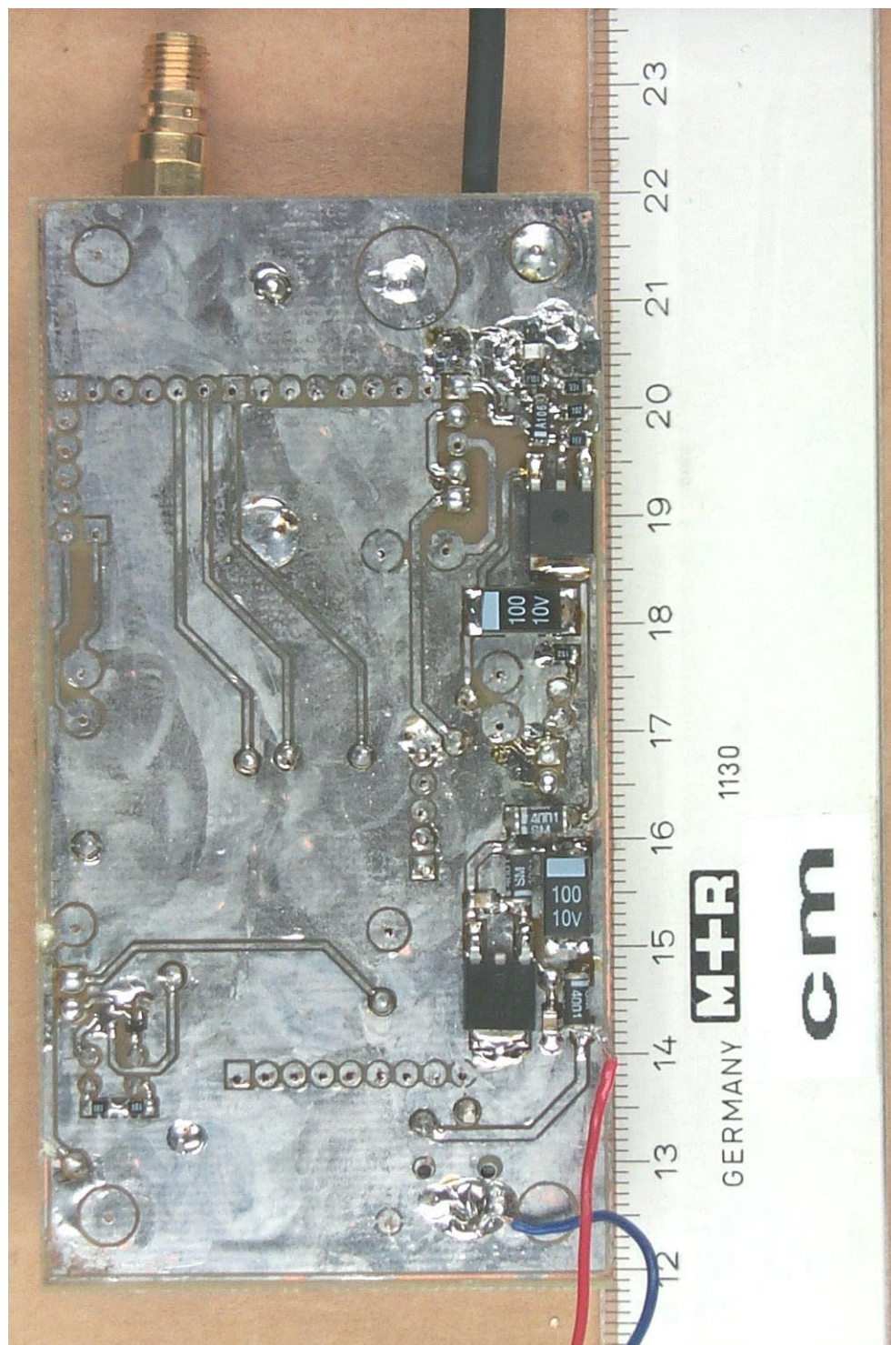
30141_4.jpg BCM001 test board, bottom view
