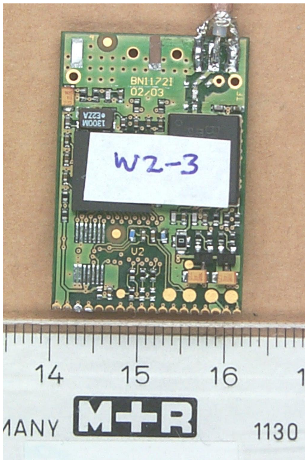
30141_7.jpg BCM001 W2-3 (with temporary antenna connector), top view
