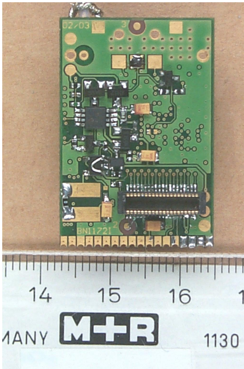
30141_6.jpg BCM001 W2-3 (with temporary antenna connector), bottom view
