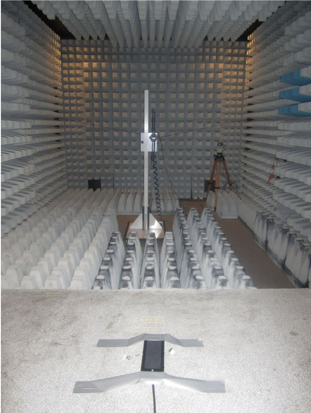
121762_3.jpg: Test setup fully anechoic chamber
