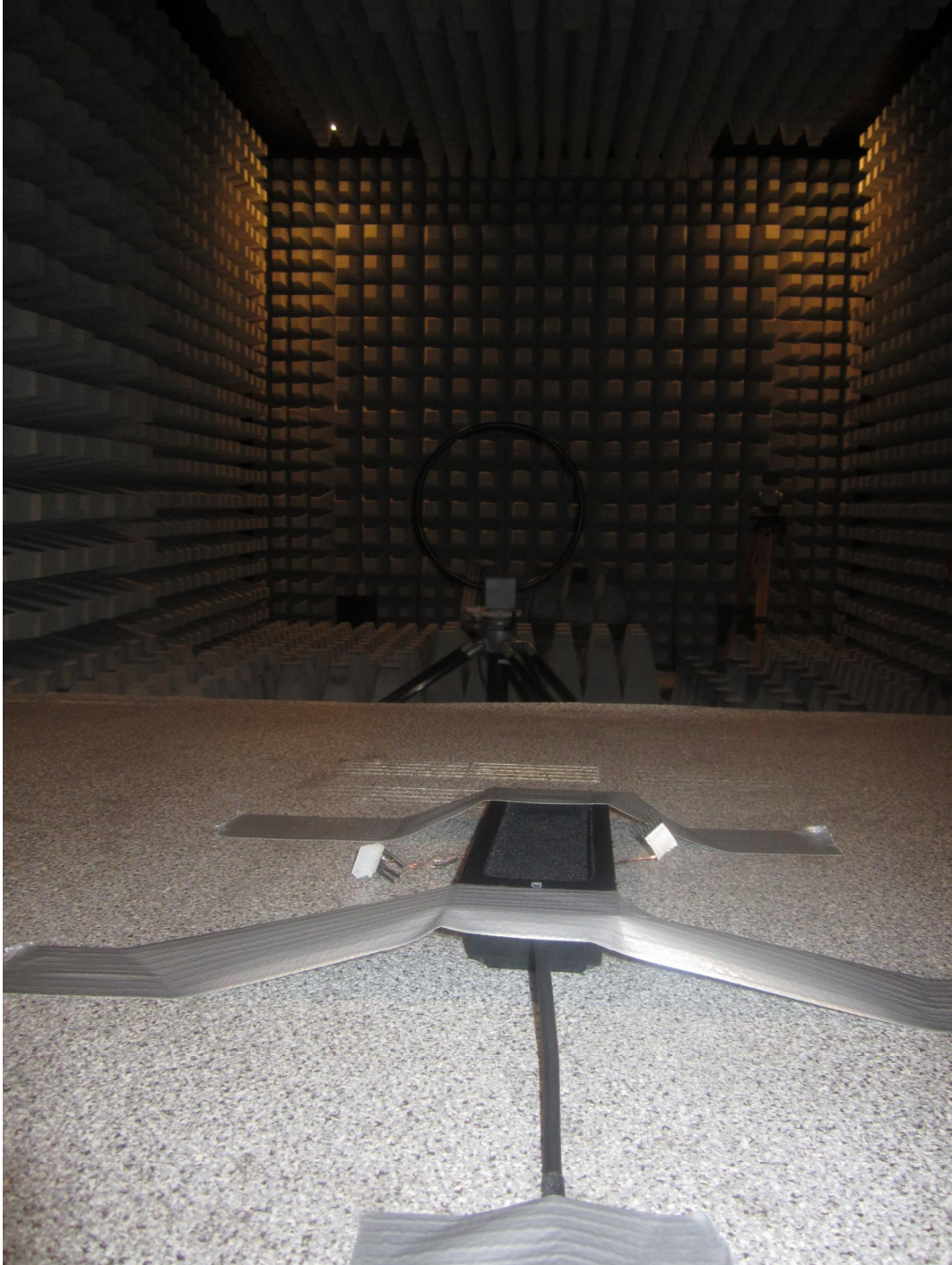
121762_1.jpg: Test setup fully anechoic chamber
