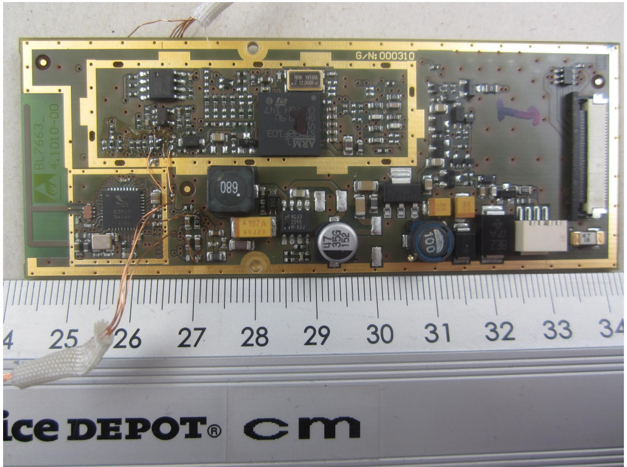
121762_9.jpg: EUT, PCB top view
