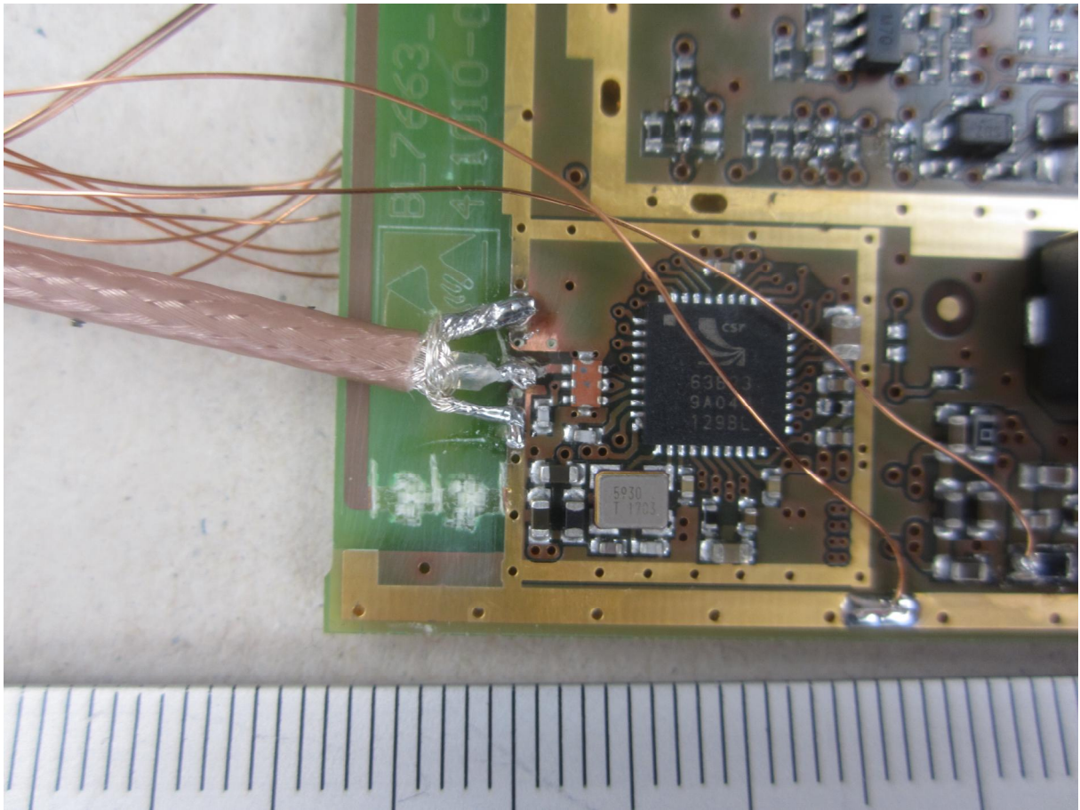
121762_11.jpg: EUT, temporary antenna connector
