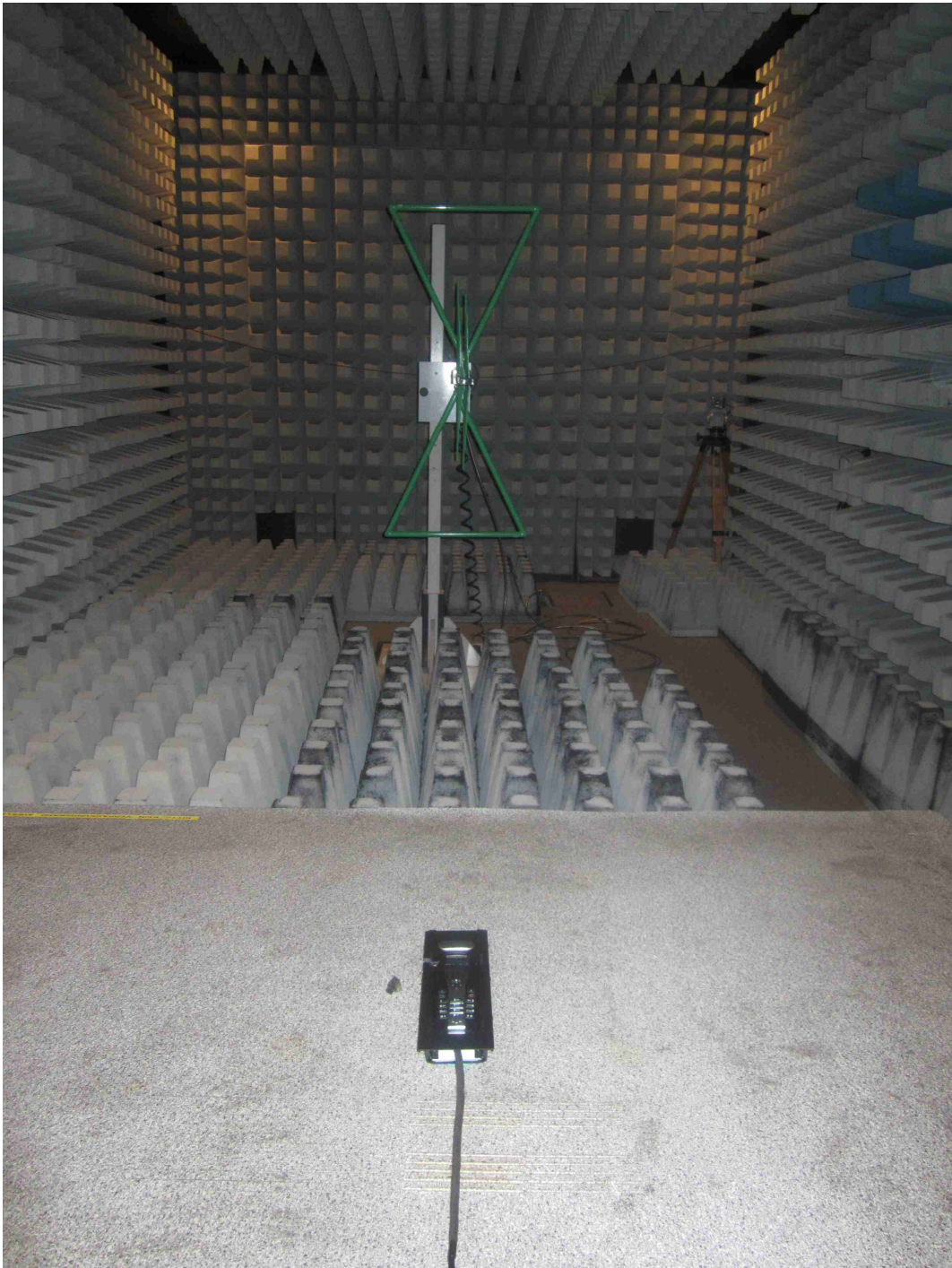
122097_03: Test setup - Radiated emission – 30 MHz – 1 GHz (fully anechoic chamber)
