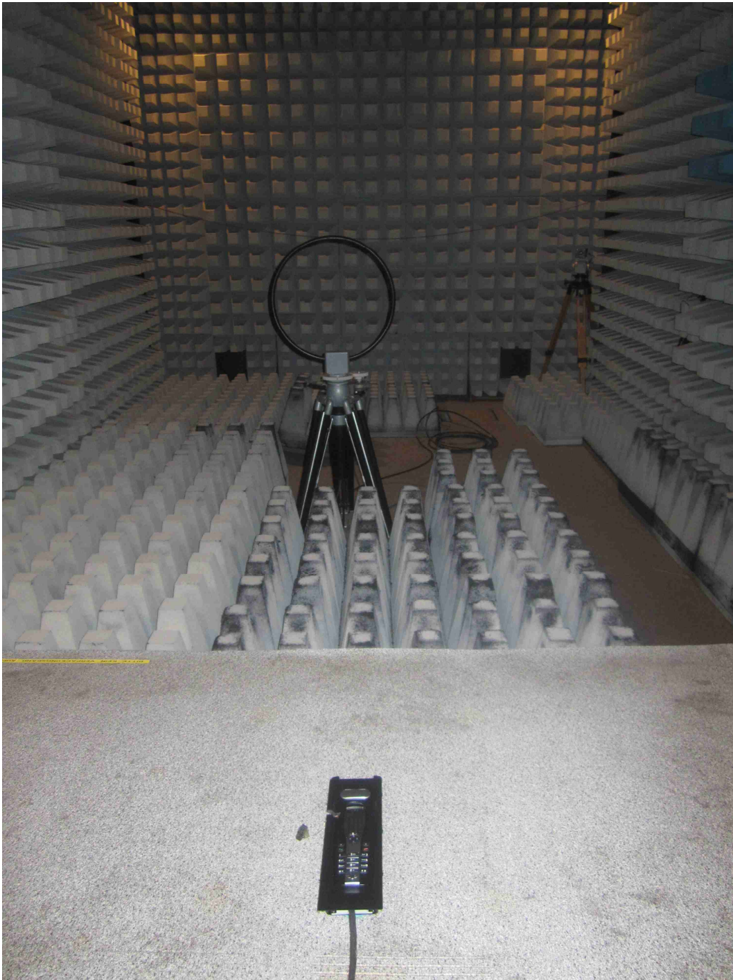
122097_02: Test setup - Radiated emission – 9 kHz – 30 MHz (fully anechoic chamber)
