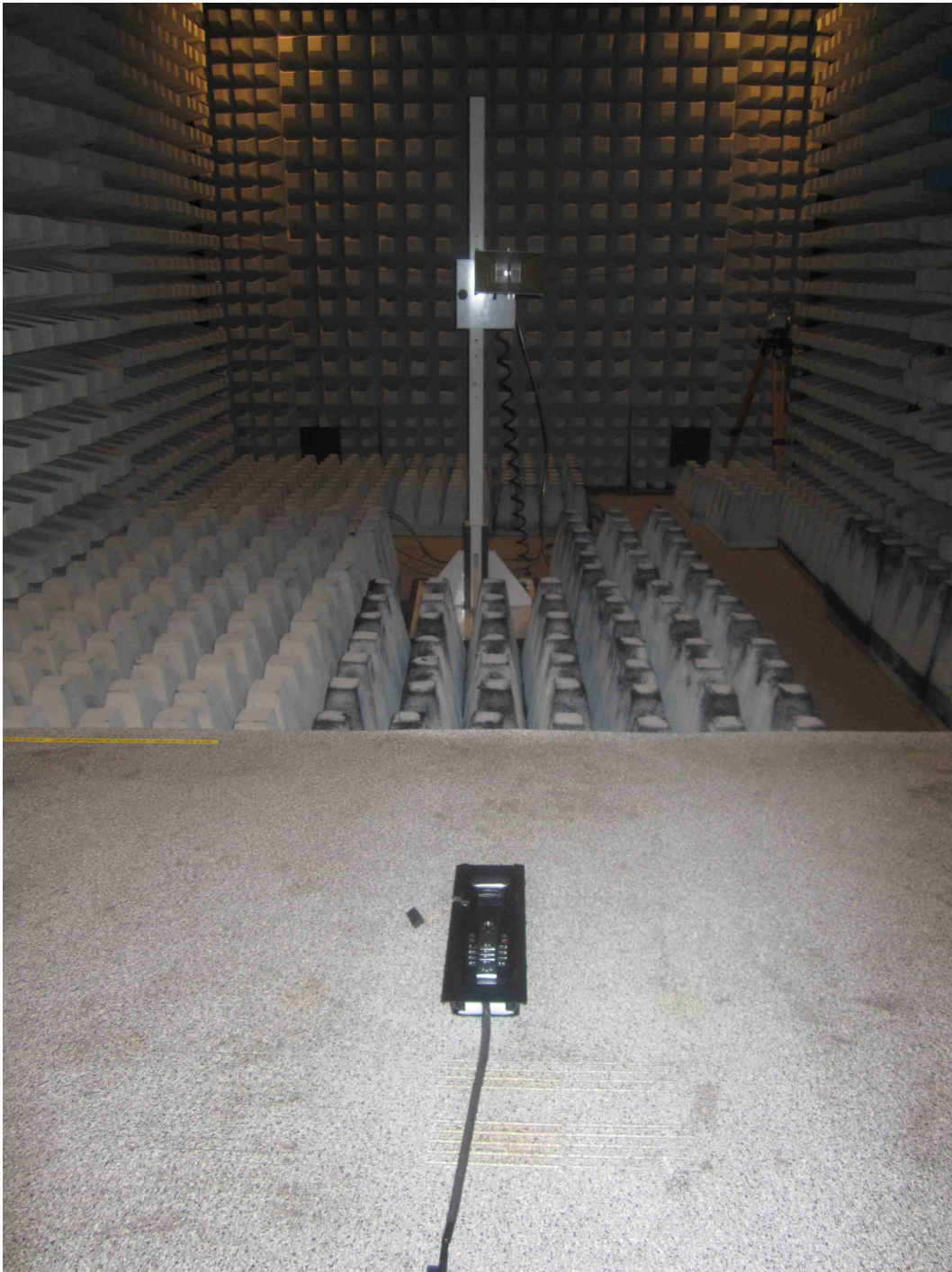
122097_01: Test setup - Radiated emission – 1 GHz – 12 GHz (fully anechoic chamber)
