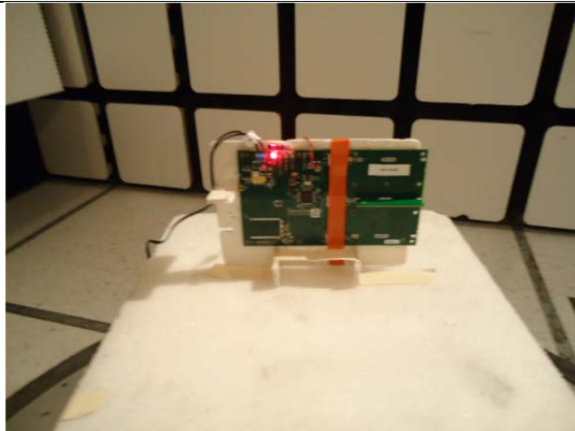
PCB Trace antenna
