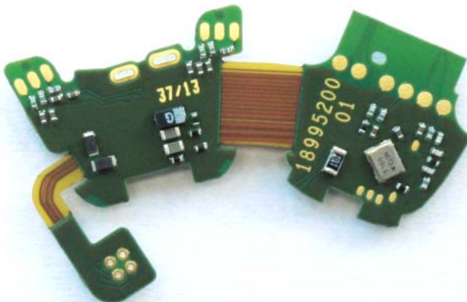
Main board, bottom side
