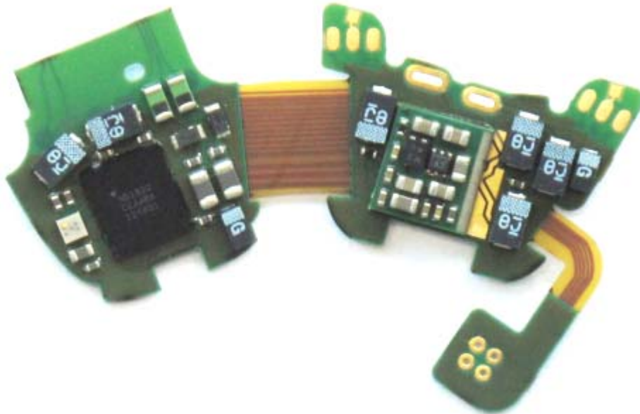
Main board, top side
