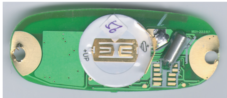
Bottom View of Printed Circuit Board
