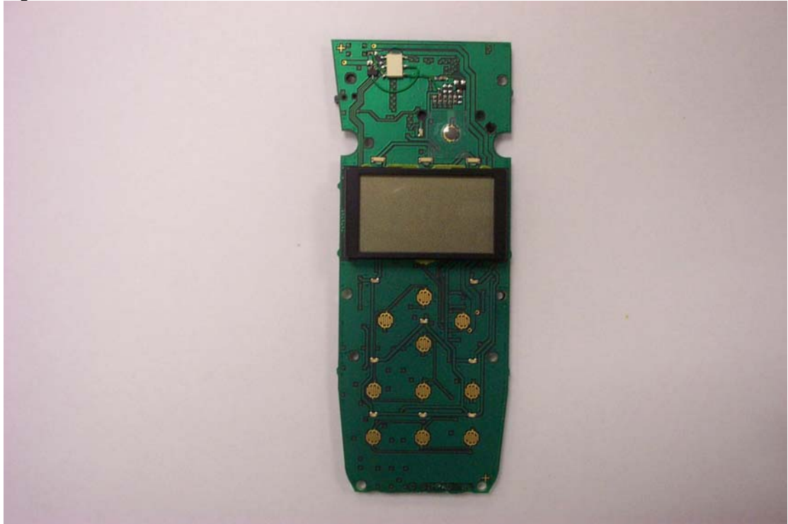
Fig 3: Rear view of AHS81 PCB
