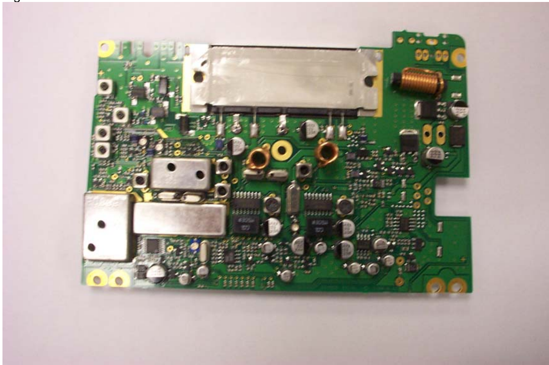
Fig 2: Reverse of RS80B RF PCB
