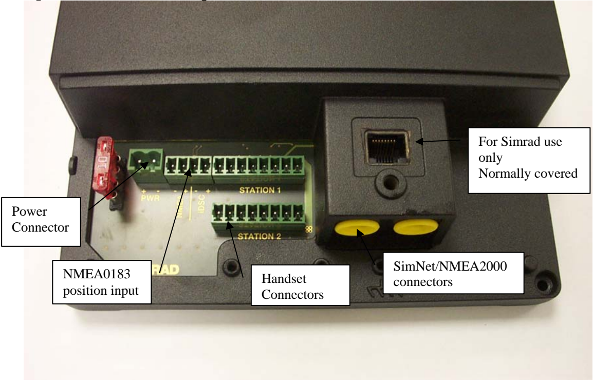
Fig 6: View of RS80B showing Connectors
