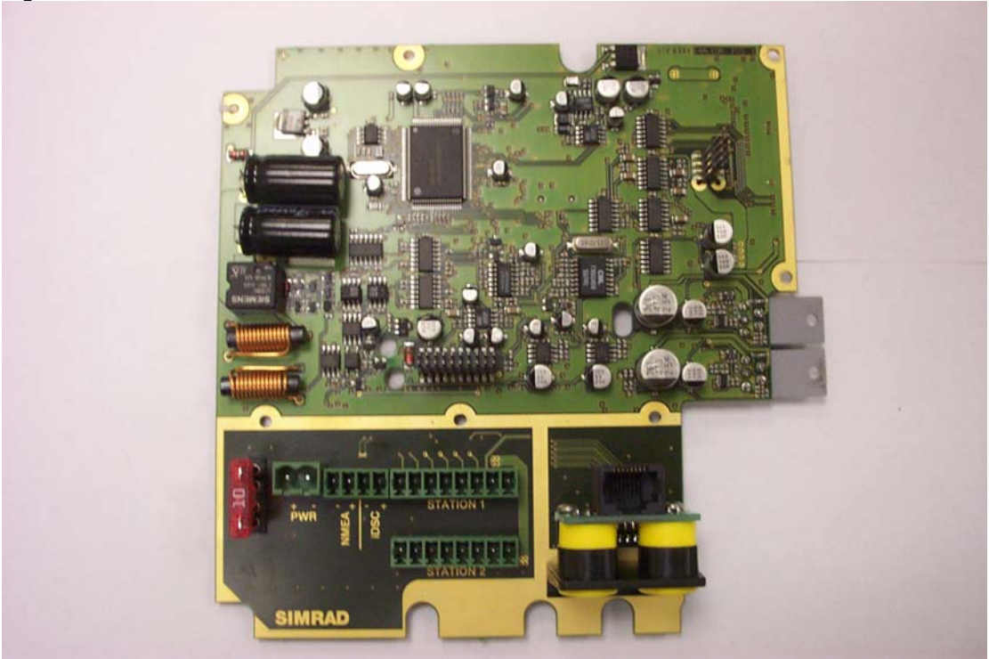
Fig 5: Reverse of RS80 Control PCB
