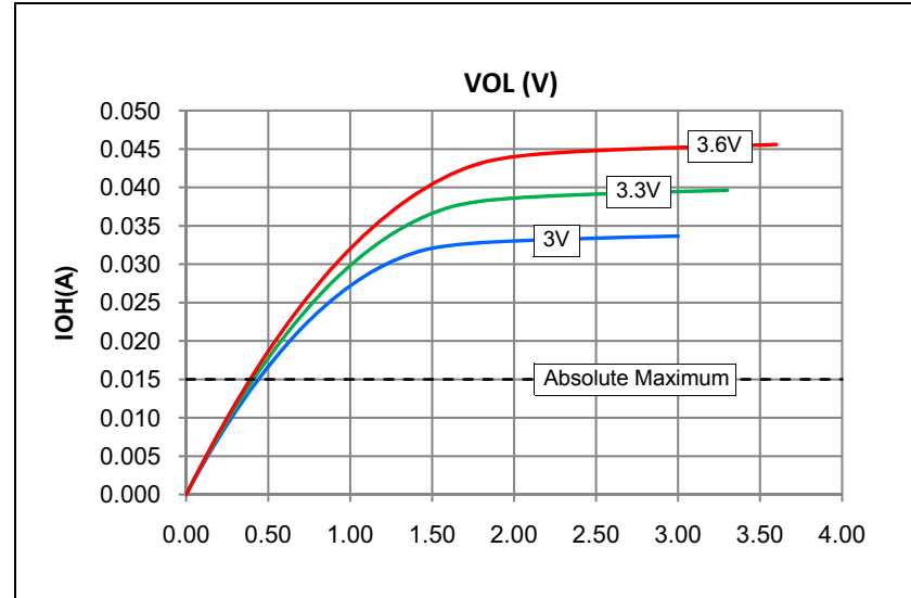
FIGURE 30-2: I/O OUTPUT VOLTAGE LOW (VOL)
