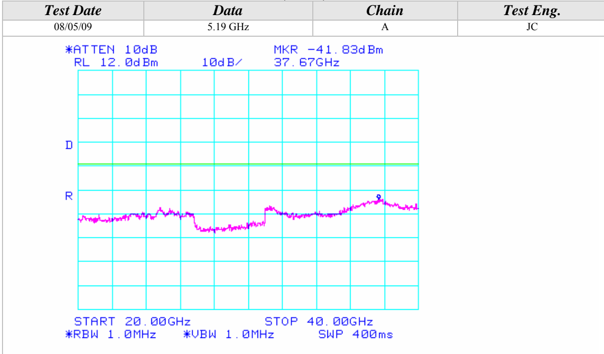
802.11n Mode, 5GHz, 40MHz Wide
