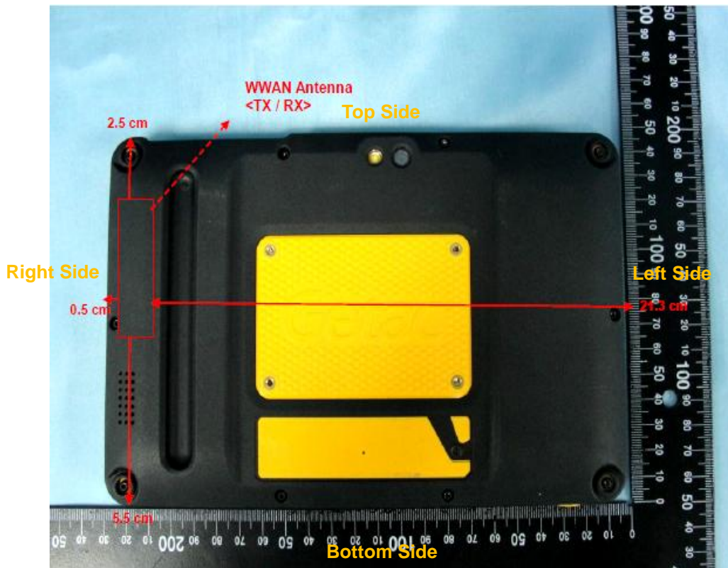
<EUT Rear View>
