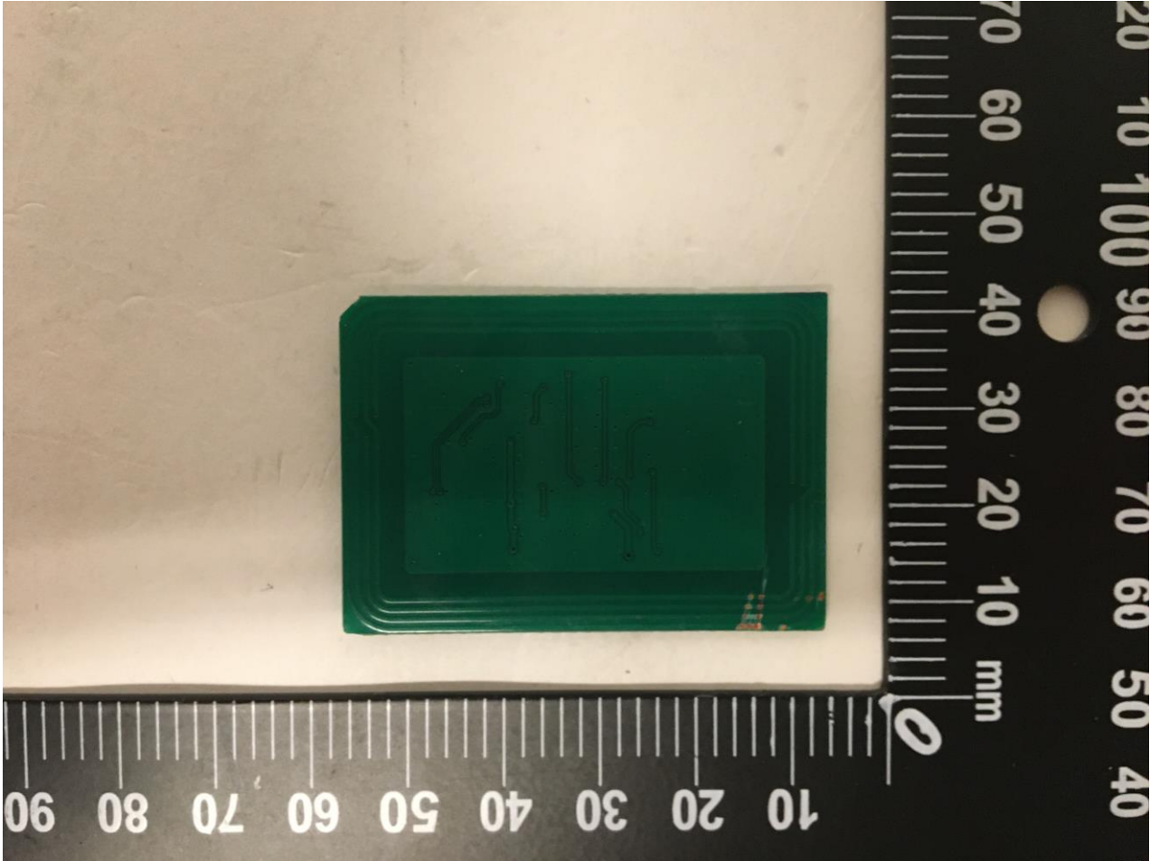
EUT: RFID Module (Brand Name: Getac / Model Name: K120 PN7462 NFC)
