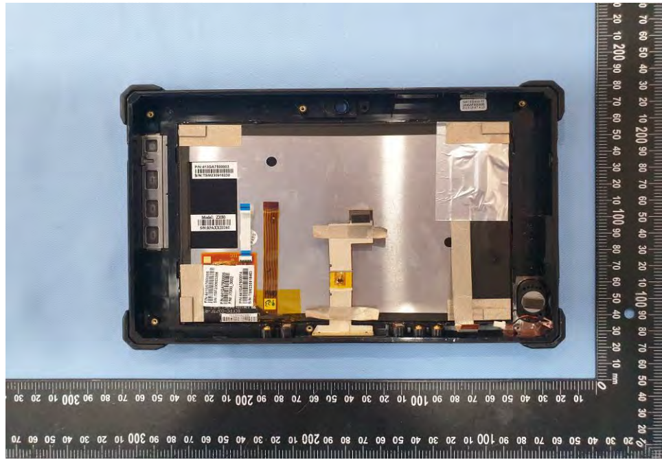
EUT Photo (80)
