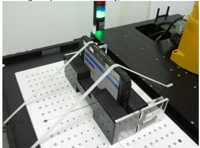
Testing Setup for Power Density, Bottom Side at 2 mm
