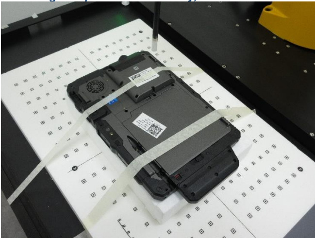
Testing Setup for Power Density, Rear Face at 2 mm
