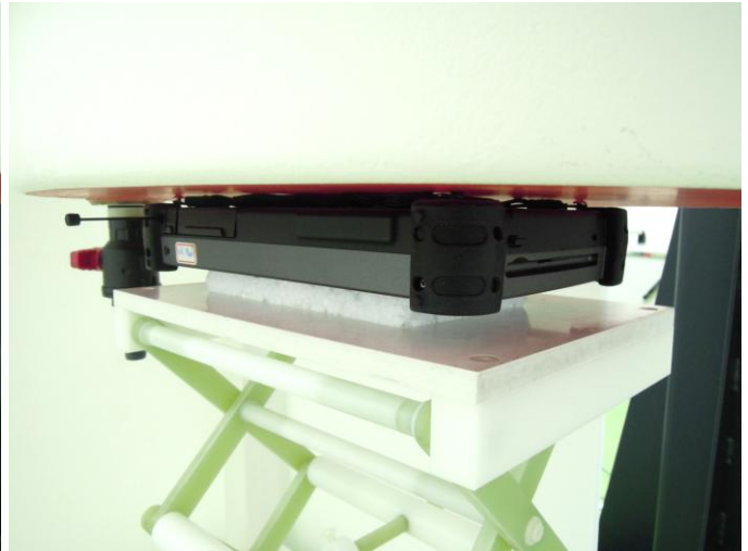
Bottom of Tablet with 0 cm Gap (Antenna Extended)
