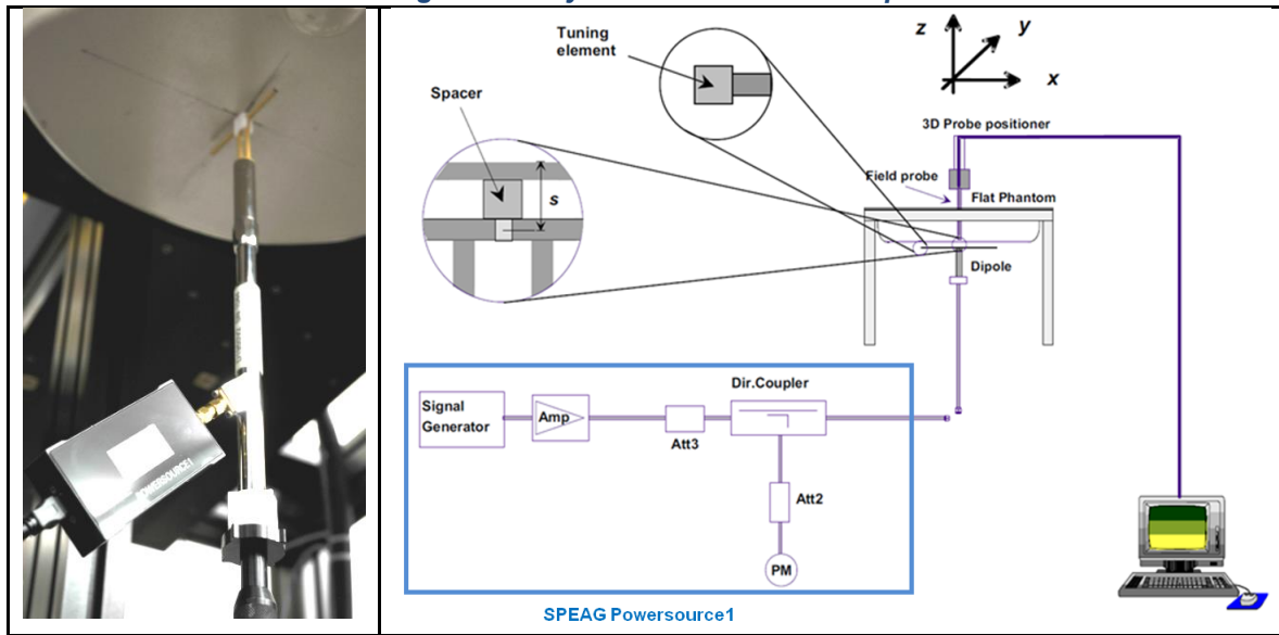
Figure 6-1: System Verification Setup
