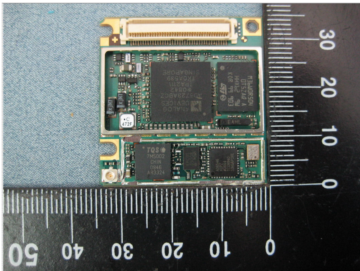
Rear View of WWAM Board-2
