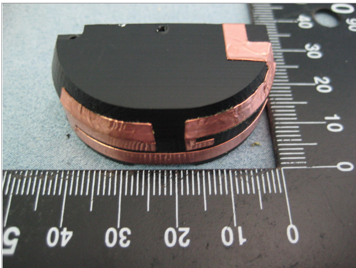
WWAN Antenna-2
