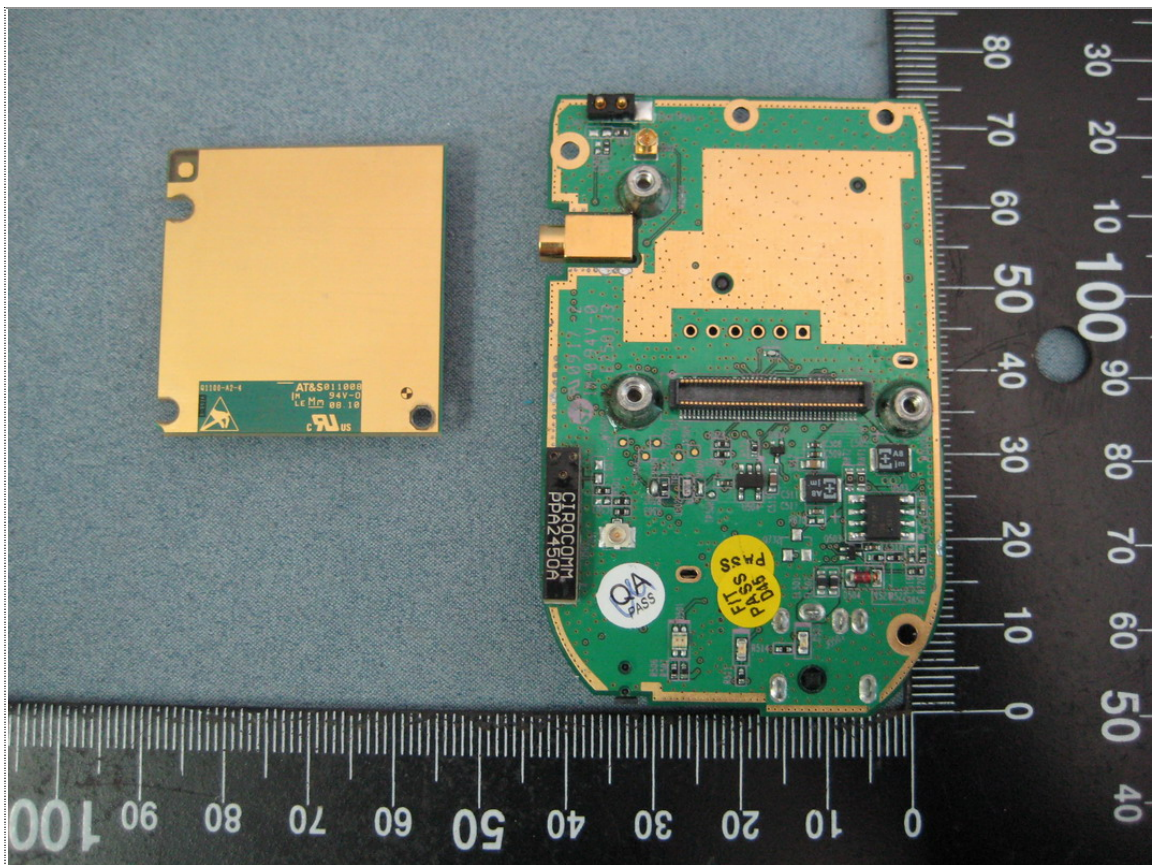
Rear View of PCB Board-3
