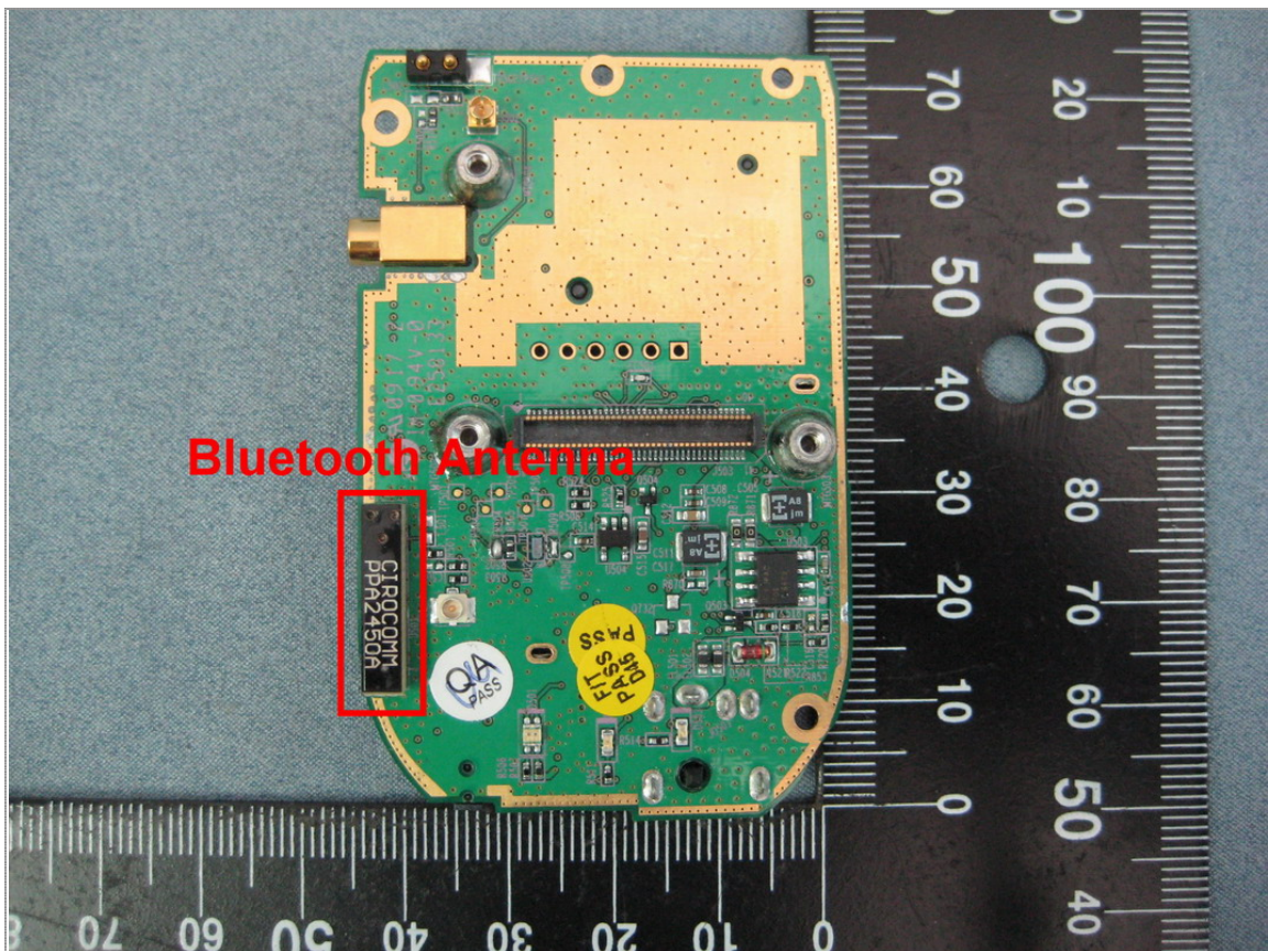
Bluetooth Antenna Location
