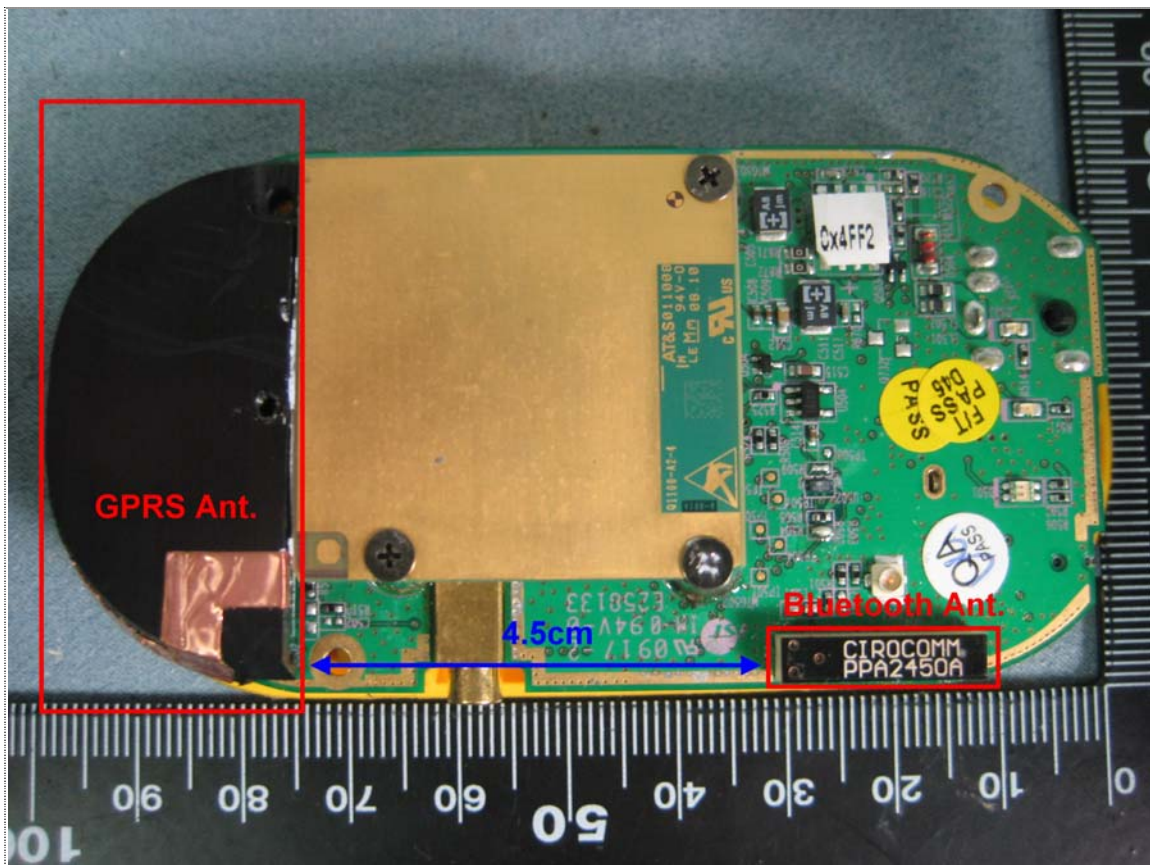
Antenna Separation
