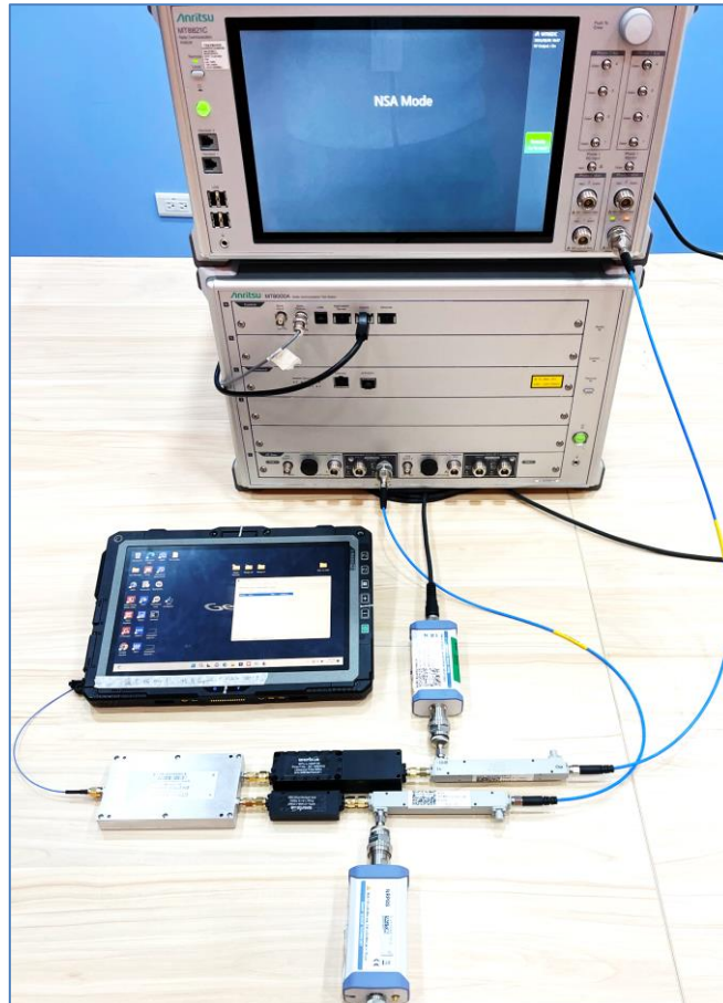
Setup for Conducted Power Testing (Figure 4-6)
