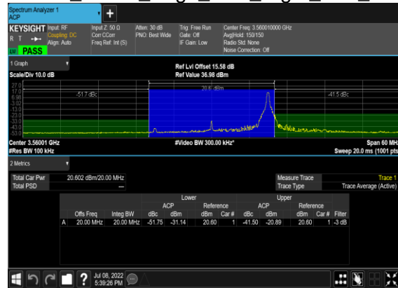
B13_N48(20M)_DFT-s-OFDM_QPSK_Edge_1RB_Right_Low_CH
