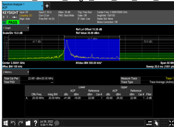
B13_N48(20M)_DFT-s-OFDM_QPSK_Edge_1RB_Left_Low_CH
