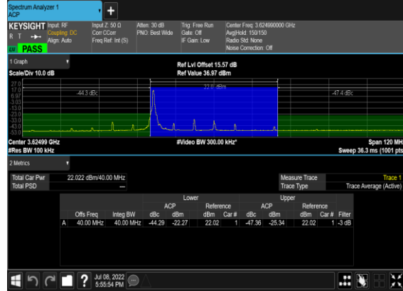
B13_N48(40M)_DFT-s-OFDM_QPSK_Outer_Full_Mid_CH
