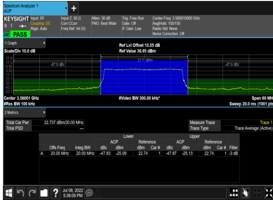
B13_N48(20M)_DFT-s-OFDM_PI_2-BPSK_Edge_1RB_Right_Low_CH
