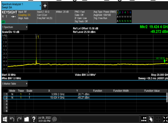
B13_N48(10M)_DFT-s-OFDM_BPSK_Edge_1RB_Right_Low_CH
