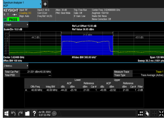
B13_N48(40M)_DFT-s-OFDM_QPSK_Edge_1RB_Right_Mid_CH
