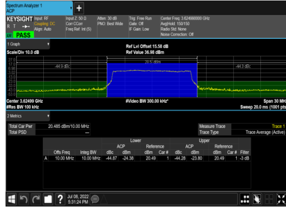
B13_N48(10M)_DFT-s-OFDM_QPSK_Edge_1RB_Right_Mid_CH
