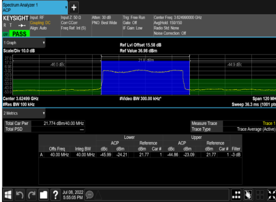
B13_N48(40M)_DFT-s-OFDM_PI_2-BPSK_Edge_1RB_Right_Mid_CH
