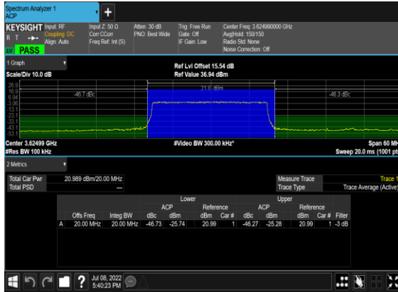
B13_N48(20M)_DFT-s-OFDM_PI_2-BPSK_Edge_1RB_Right_Mid_CH
