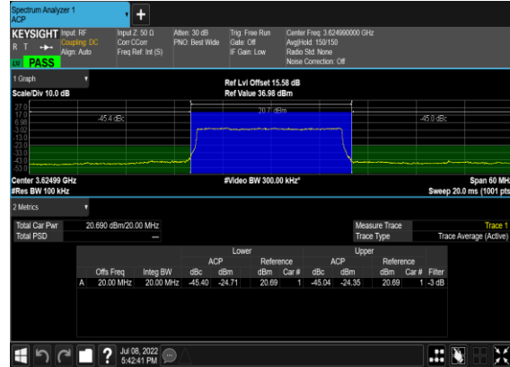
B13_N48(20M)_DFT-s-OFDM_QPSK_Edge_1RB_Right_Mid_CH
