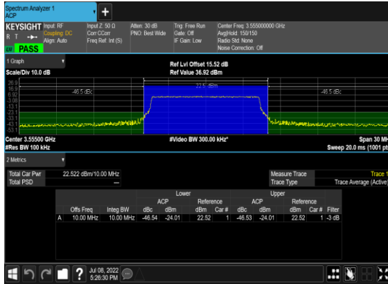
B13_N48(10M)_DFT-s-OFDM_PI_2-BPSK_Edge_1RB_Right_Low_CH
