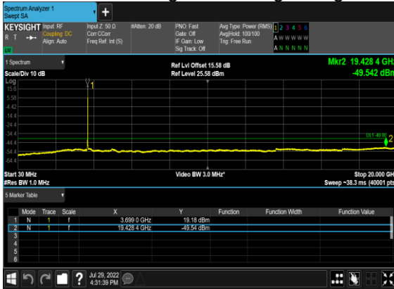
B13_N48(20M)_DFT-s-OFDM_BPSK_Edge_1RB_Right_High_CH
