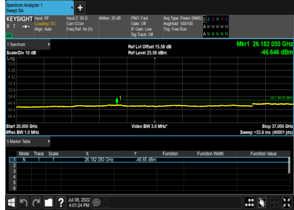
B13_N48(10M)_DFT-s-OFDM_BPSK_Outer_Full_Mid_CH
