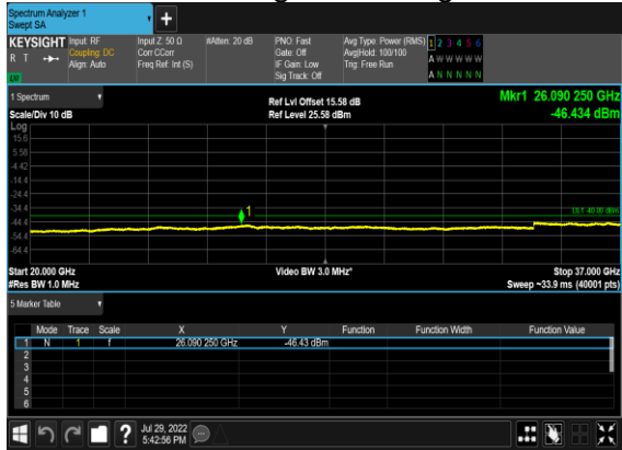
B13_N48(40M)_DFT-s-OFDM_BPSK_Outer_Full_Mid_CH
