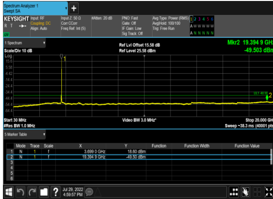
B13_N48(40M)_DFT-s-OFDM_BPSK_Outer_Full_High_CH
