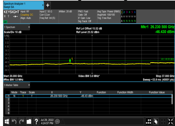
B13_N48(20M)_DFT-s-OFDM_BPSK_Outer_Full_Mid_CH
