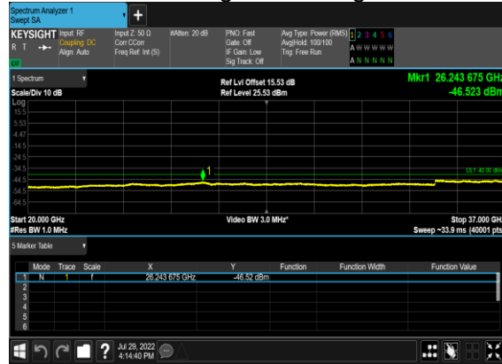
B13_N48(20M)_DFT-s-OFDM_BPSK_Edge_1RB_Right_Low_CH
