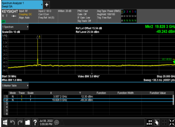
B13_N48(10M)_DFT-s-OFDM_QPSK_Outer_Full_Low_CH
