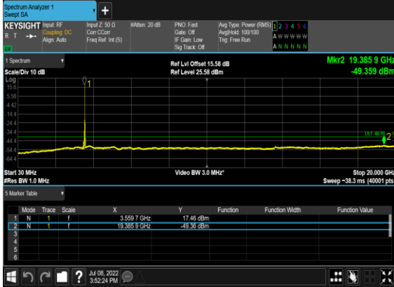
B13_N48(10M)_DFT-s-OFDM_BPSK_Outer_Full_Low_CH
