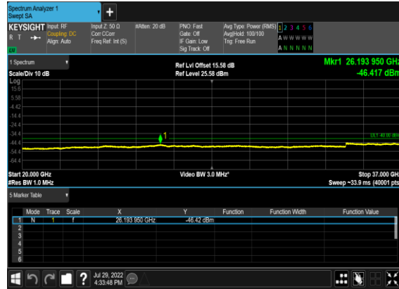
B13_N48(20M)_DFT-s-OFDM_BPSK_Outer_Full_High_CH
