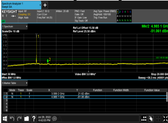
B13_N48(40M)_DFT-s-OFDM_BPSK_Outer_Full_Low_CH
