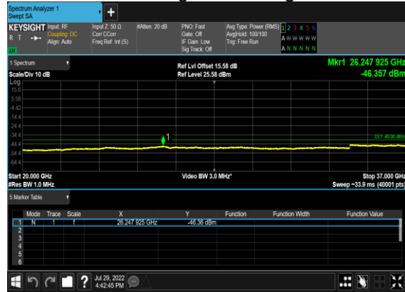
B13_N48(40M)_DFT-s-OFDM_BPSK_Outer_Full_Low_CH
