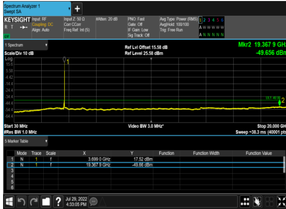
B13_N48(20M)_DFT-s-OFDM_BPSK_Outer_Full_High_CH
