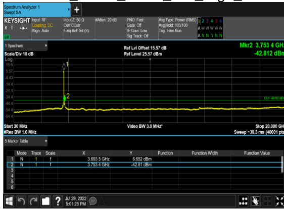
B13_N48(40M)_DFT-s-OFDM_QPSK_Outer_Full_High_CH
