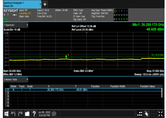
B13_N48(10M)_DFT-s-OFDM_BPSK_Outer_Full_Low_CH
