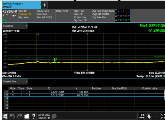
B13_N48(10M)_DFT-s-OFDM_BPSK_Edge_1RB_Right_Mid_CH
