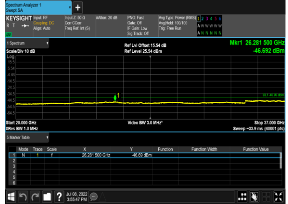
B13_N48(10M)_DFT-s-OFDM_QPSK_Outer_Full_Low_CH
