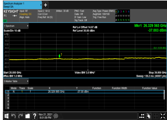
B5_N77(20M)_DFT-s-OFDM_BPSK_Edge_1RB_Left_Mid_CH
