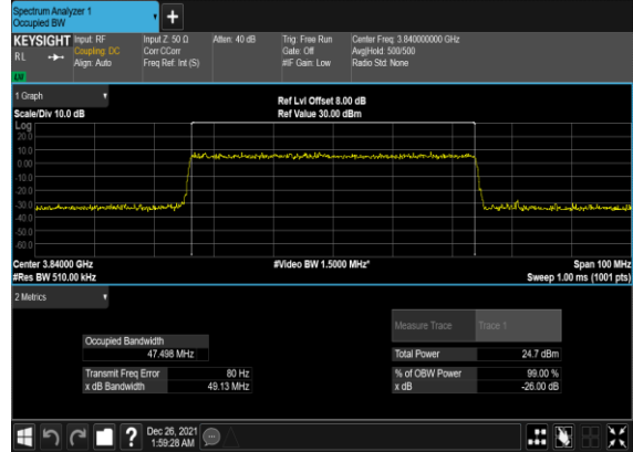
B5_N77(50M)_CP-OFDM_16 QAM_Outer_Full_Mid_CH
