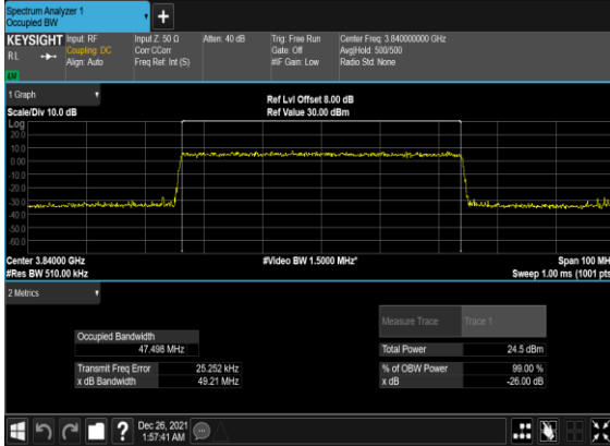
B5_N77(50M)_CP-OFDM_QPSK_Outer_Full_Mid_CH
