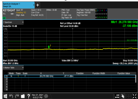
B5_N77(20M)_DFT-s-OFDM_QPSK_Edge_1RB_Left_Mid_CH
