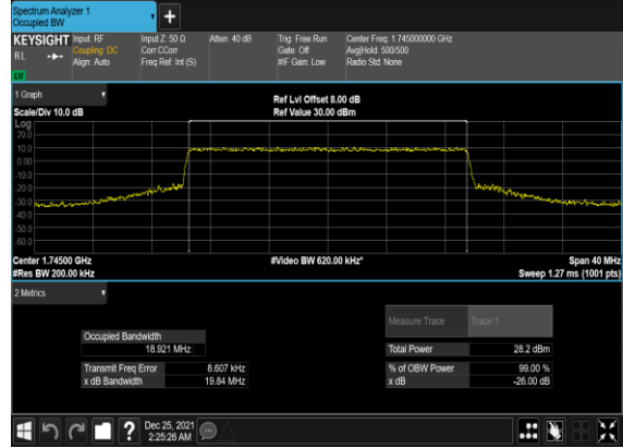
B13_N66(20M)_CP-OFDM_16QAM_Outer_Full_Mid_CH
