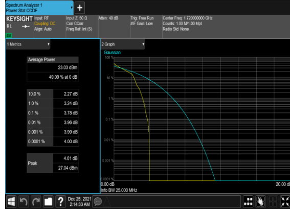
B13_N66(20M)_DFT-s-OFDM_PI_2-BPSK_Edge_1RB_Left_Low_CH
