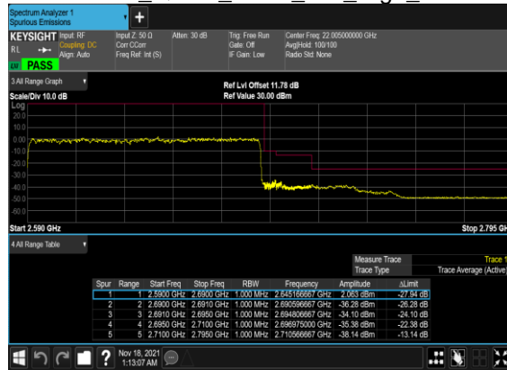
B4_N41(100M)_DFT-s-OFDM_QPSK_Outer_Full_High_CH
