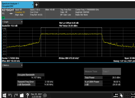
B13_N66(15M)_CP- OFDM_QPSK_Outer_Full_Mid_CH
