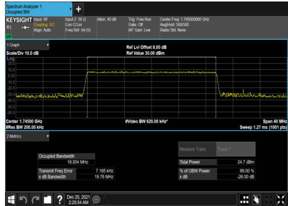
B13_N66(20M)_CP-OFDM_256QAM_Outer_Full_Mid_CH
