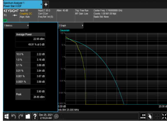
B13_N66(20M)_DFT-s-OFDM_PI_2-BPSK_Edge_1RB_Left_Mid_CH
