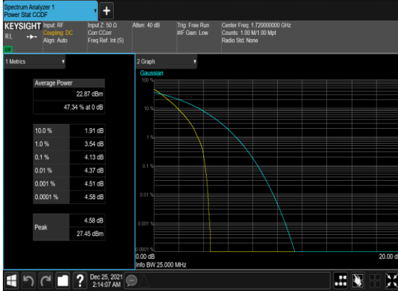
B13_N66(20M)_DFT-s-OFDM_PI_2-BPSK_Outer_Full_Low_CH
