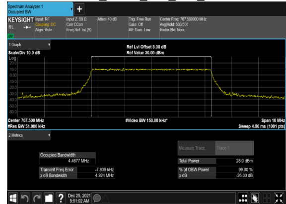
B2_N12(5M)_CP-OFDM_16QAM_Outer_Full_Mid_CH
