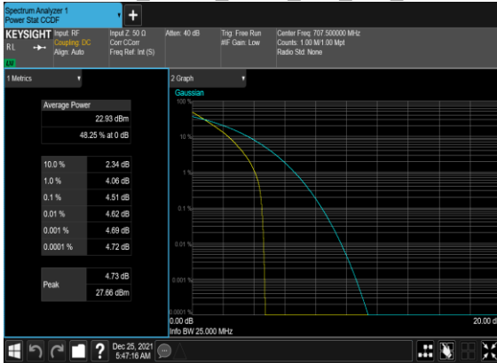
B2_N12(10M)_DFT-s-OFDM_QPSK_Outer_Full_Mid_CH
