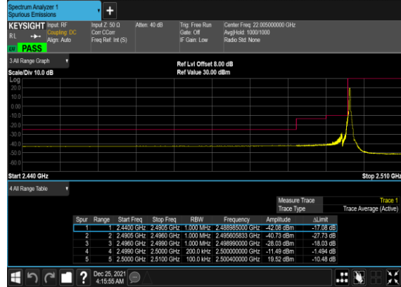
B5_N7(10M)_DFT-s-OFDM_QPSK_Edge_1RB_Left_Low_CH
