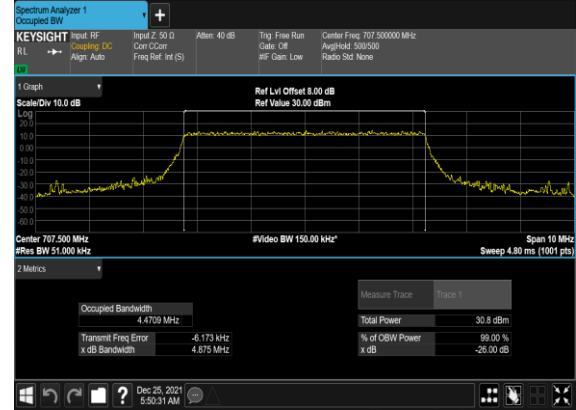
B2_N12(5M)_DFT-s-OFDM_QPSK_Outer_Full_Mid_CH
