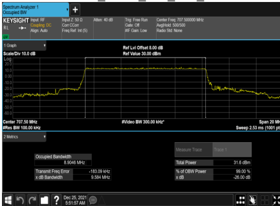
B2_N12(10M)_DFT-s-OFDM_PI_2- BPSK_Outer_Full_Mid_CH
