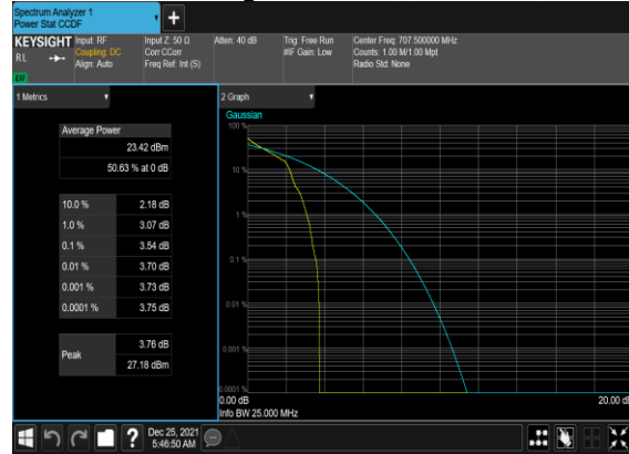
B2_N12(10M)_DFT-s-OFDM_PI_2-BPSK_Edge_1RB_Left_Mid_CH
