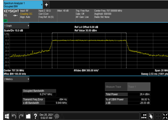
B2_N12(10M)_CP-OFDM_16QAM_Outer_Full_Mid_CH
