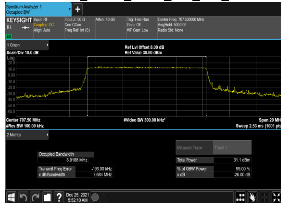
B2_N12(10M)_DFT-s- OFDM_QPSK_Outer_Full_Mid_CH
