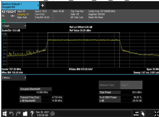
B2_N12(15M)_CP-OFDM_QPSK_Outer_Full_Mid_CH
