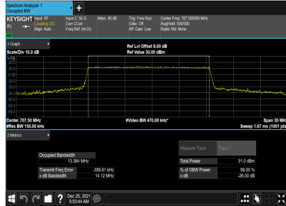
B2_N12(15M)_DFT-s-OFDM_QPSK_Outer_Full_Mid_CH
