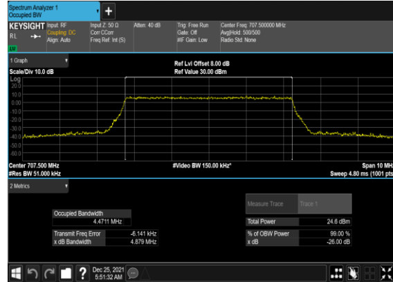
B2_N12(5M)_CP-OFDM_256 QAM_Outer_Full_Mid_CH
