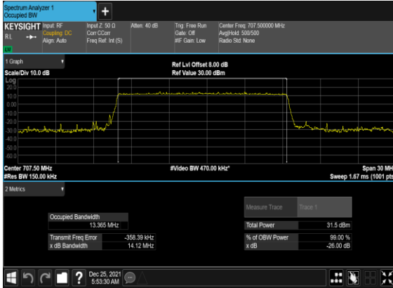
B2_N12(15M)_DFT-s-OFDM_PI_2-BPSK_Outer_Full_Mid_CH
