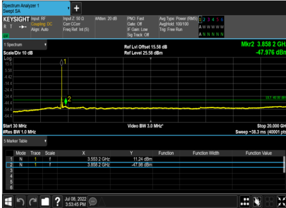
B13_N48(10M)_DFT-s-OFDM_QPSK_Outer_Full_Low_CH
