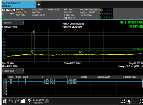
B13_N48(40M)_DFT-s-OFDM_QPSK_Outer_Full_Mid_CH
