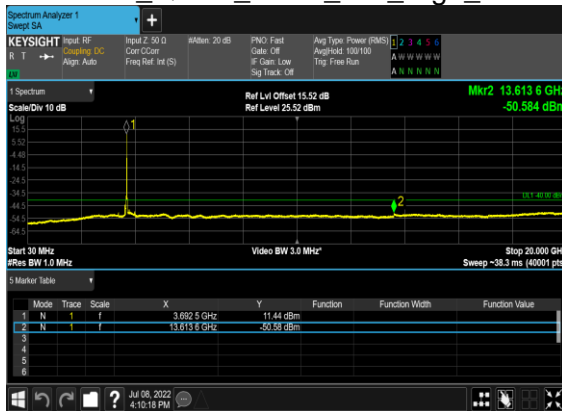
B13_N48(10M)_DFT-s-OFDM_QPSK_Outer_Full_High_CH
