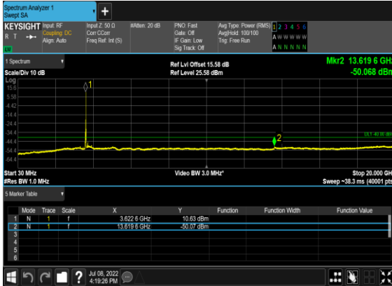
B13_N48(10M)_DFT-s-OFDM_QPSK_Outer_Full_Mid_CH
