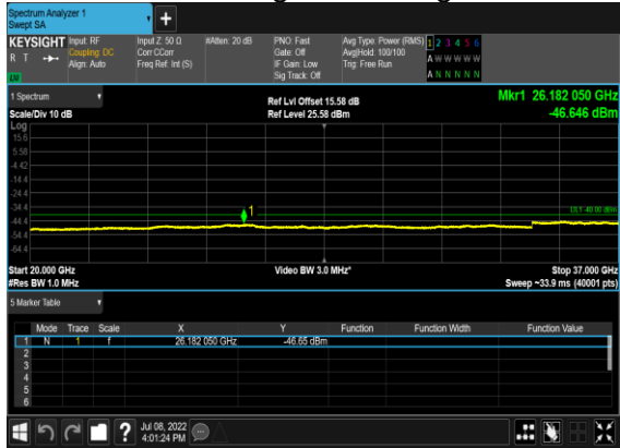
B13_N48(10M)_DFT-s-OFDM_BPSK_Outer_Full_Mid_CH
