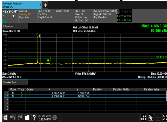
B13_N48(40M)_DFT-s-OFDM_BPSK_Outer_Full_Mid_CH
