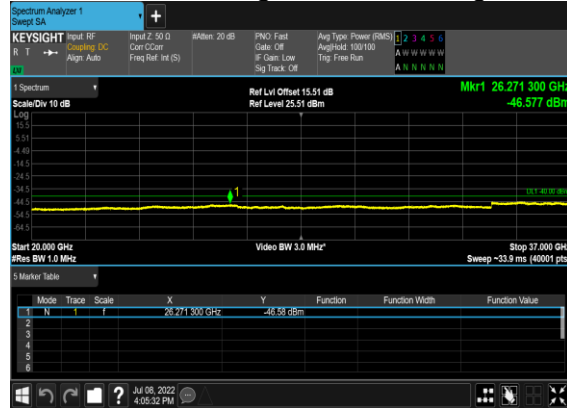
B13_N48(10M)_DFT-s-OFDM_BPSK_Edge_1RB_Right_High_CH
