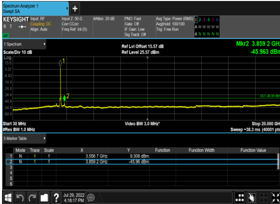
B13_N48(20M)_DFT-s-OFDM_QPSK_Outer_Full_Low_CH
