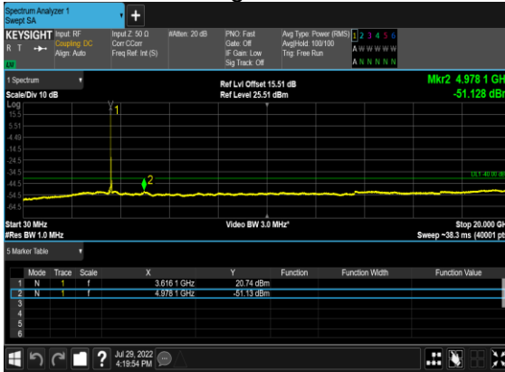
B13_N48(20M)_DFT-s-OFDM_QPSK_Edge_1RB_Left_Mid_CH
