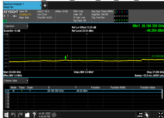
B13_N48(40M)_DFT-s-OFDM_QPSK_Outer_Full_Low_CH
