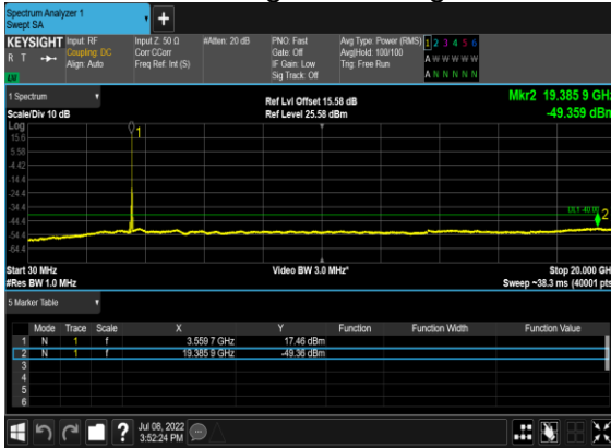
B13_N48(10M)_DFT-s-OFDM_BPSK_Outer_Full_Low_CH
