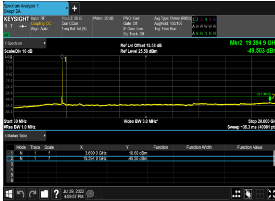
B13_N48(40M)_DFT-s-OFDM_BPSK_Outer_Full_High_CH
