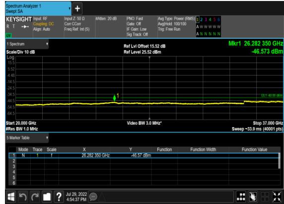
B13_N48(40M)_DFT-s-OFDM_QPSK_Outer_Full_Mid_CH
