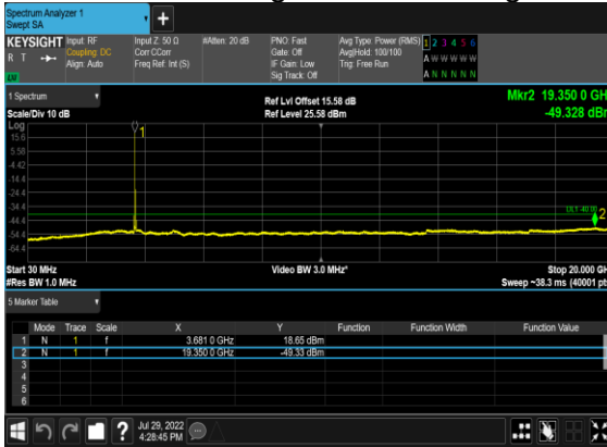
B13_N48(20M)_DFT-s-OFDM_QPSK_Edge_1RB_Left_High_CH
