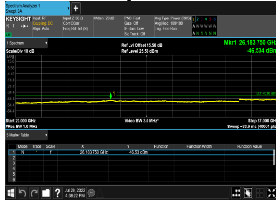
B13_N48(40M)_DFT-s-OFDM_QPSK_Edge_1RB_Left_Low_CH
