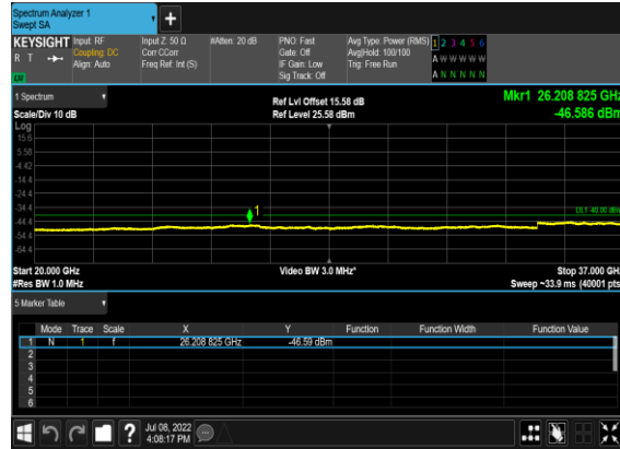
B13_N48(10M)_DFT-s-OFDM_BPSK_Outer_Full_High_CH
