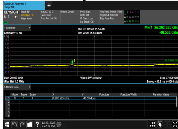
B13_N48(40M)_DFT-s-OFDM_QPSK_Edge_1RB_Left_Mid_CH
