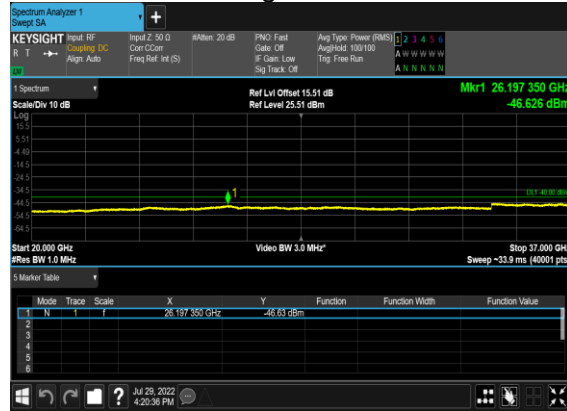
B13_N48(20M)_DFT-s-OFDM_QPSK_Edge_1RB_Left_Mid_CH
