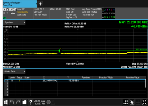
B13_N48(20M)_DFT-s-OFDM_BPSK_Outer_Full_Mid_CH
