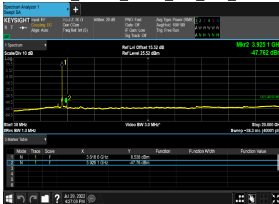
B13_N48(20M)_DFT-s-OFDM_QPSK_Outer_Full_Mid_CH
