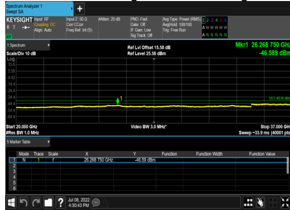
B13_N48(10M)_DFT-s-OFDM_QPSK_Edge_1RB_Left_High_CH
