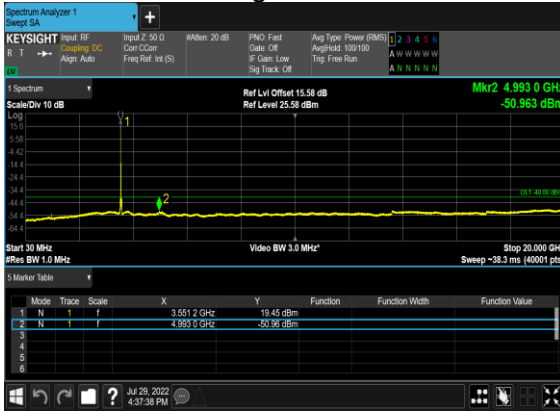
B13_N48(40M)_DFT-s-OFDM_QPSK_Edge_1RB_Left_Low_CH
