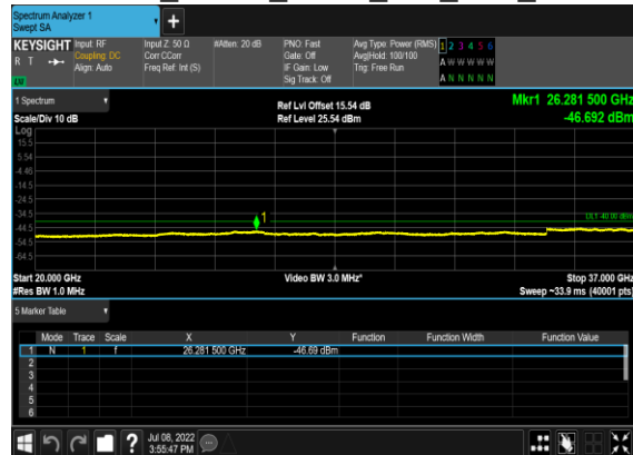
B13_N48(10M)_DFT-s-OFDM_QPSK_Outer_Full_Low_CH
