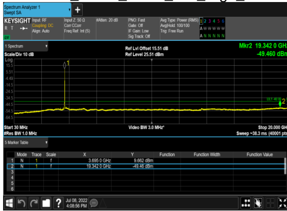
B13_N48(10M)_DFT-s-OFDM_QPSK_Outer_Full_High_CH
