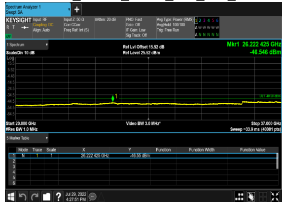
B13_N48(20M)_DFT-s-OFDM_QPSK_Outer_Full_Mid_CH
