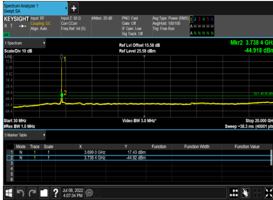
B13_N48(10M)_DFT-s-OFDM_BPSK_Outer_Full_High_CH
