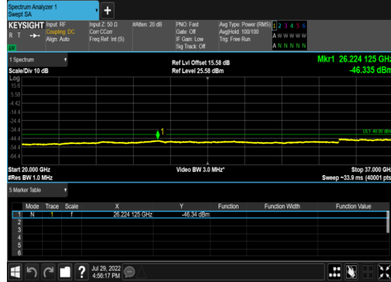
B13_N48(40M)_DFT-s-OFDM_QPSK_Edge_1RB_Left_High_CH
