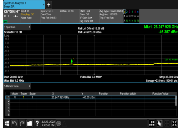
B13_N48(40M)_DFT-s-OFDM_BPSK_Outer_Full_Low_CH
