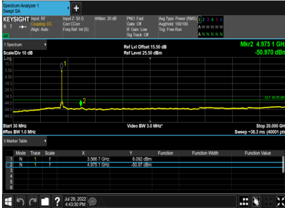
B13_N48(40M)_DFT-s-OFDM_QPSK_Outer_Full_Low_CH
