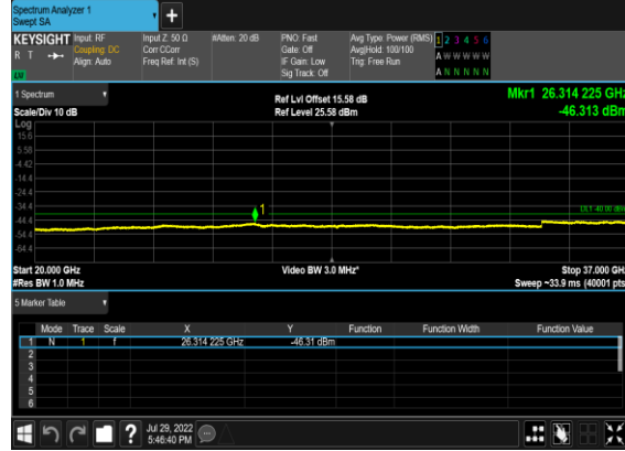
B13_N48(40M)_DFT-s-OFDM_BPSK_Edge_1RB_Right_High_CH
