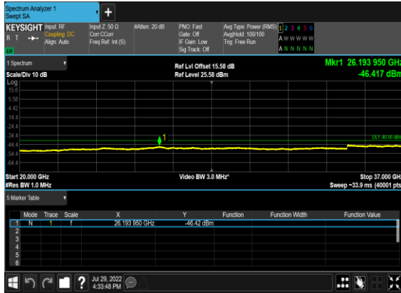
B13_N48(20M)_DFT-s-OFDM_QPSK_Edge_1RB_Right_High_C H
