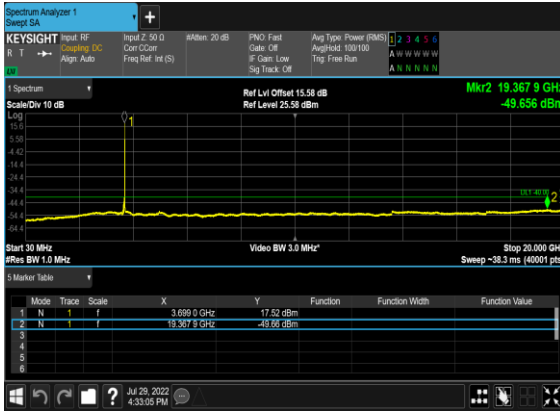
B13_N48(20M)_DFT-s-OFDM_QPSK_Edge_1RB_Right_High_C H
