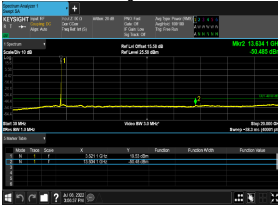
B13_N48(10M)_DFT-s-OFDM_QPSK_Edge_1RB_Left_Mid_CH
