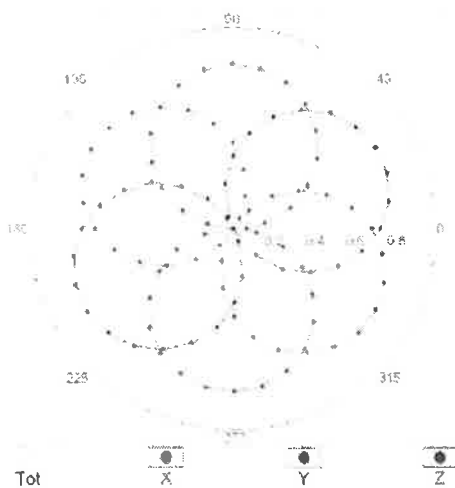
f=600 MHz,TEM
