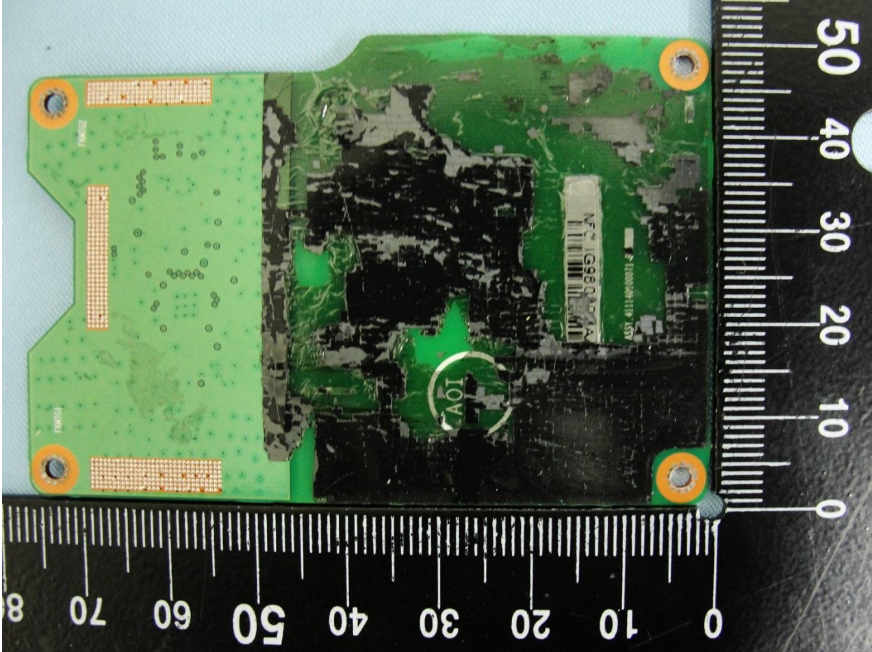
EUT: RFID module (Brand Name: Getac / Model Name: TRF7970A)
