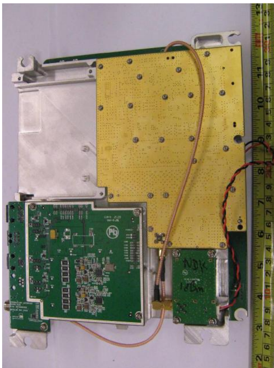
Internal View 2
