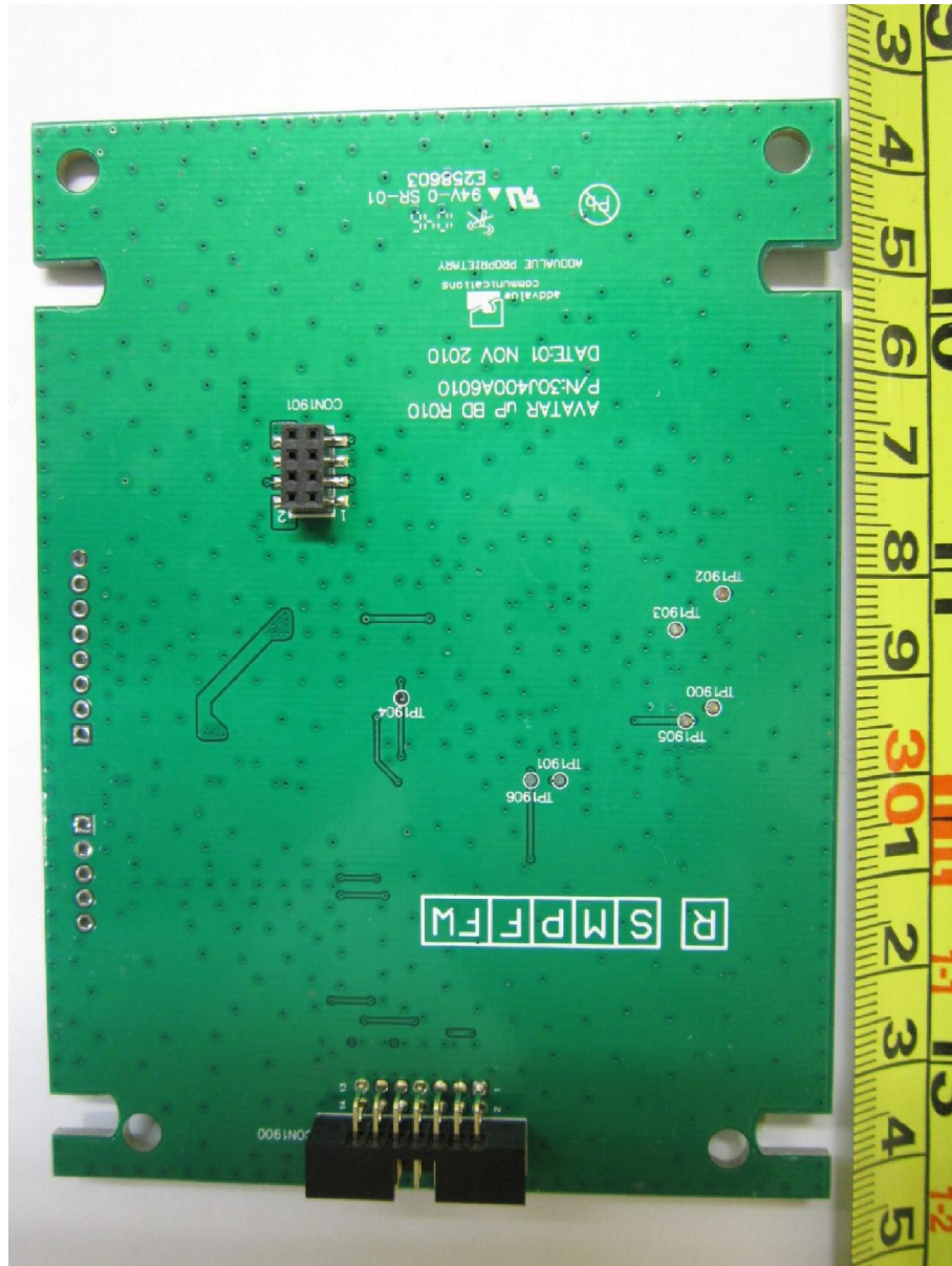
Microprocessor PCB Trace Side
