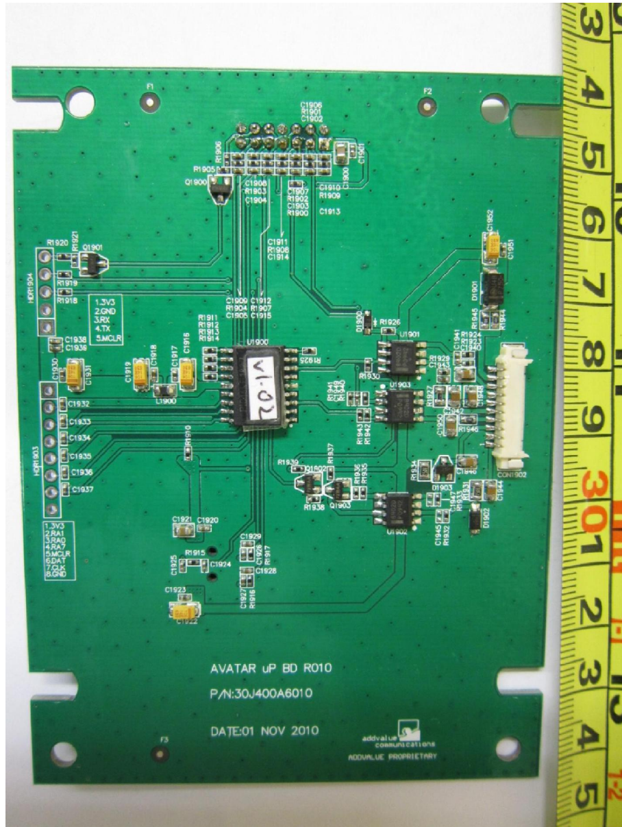
Microprocessor PCB Component Side
