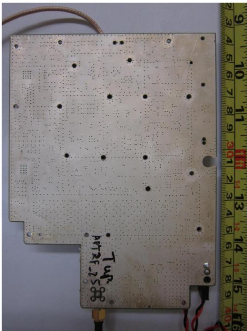
Base Band PCB Trace Side
