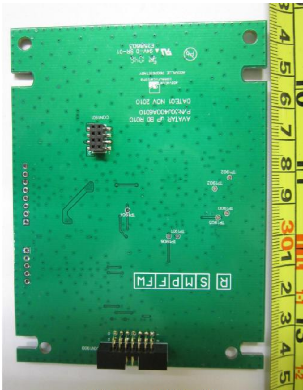
Microprocessor PCB Trace Side
