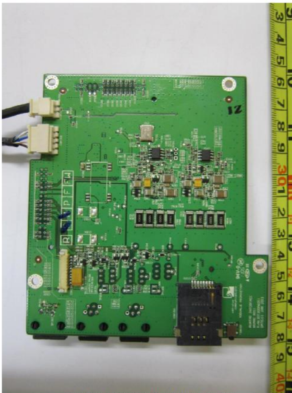
Interface Connecting Board PCB Trace Side
