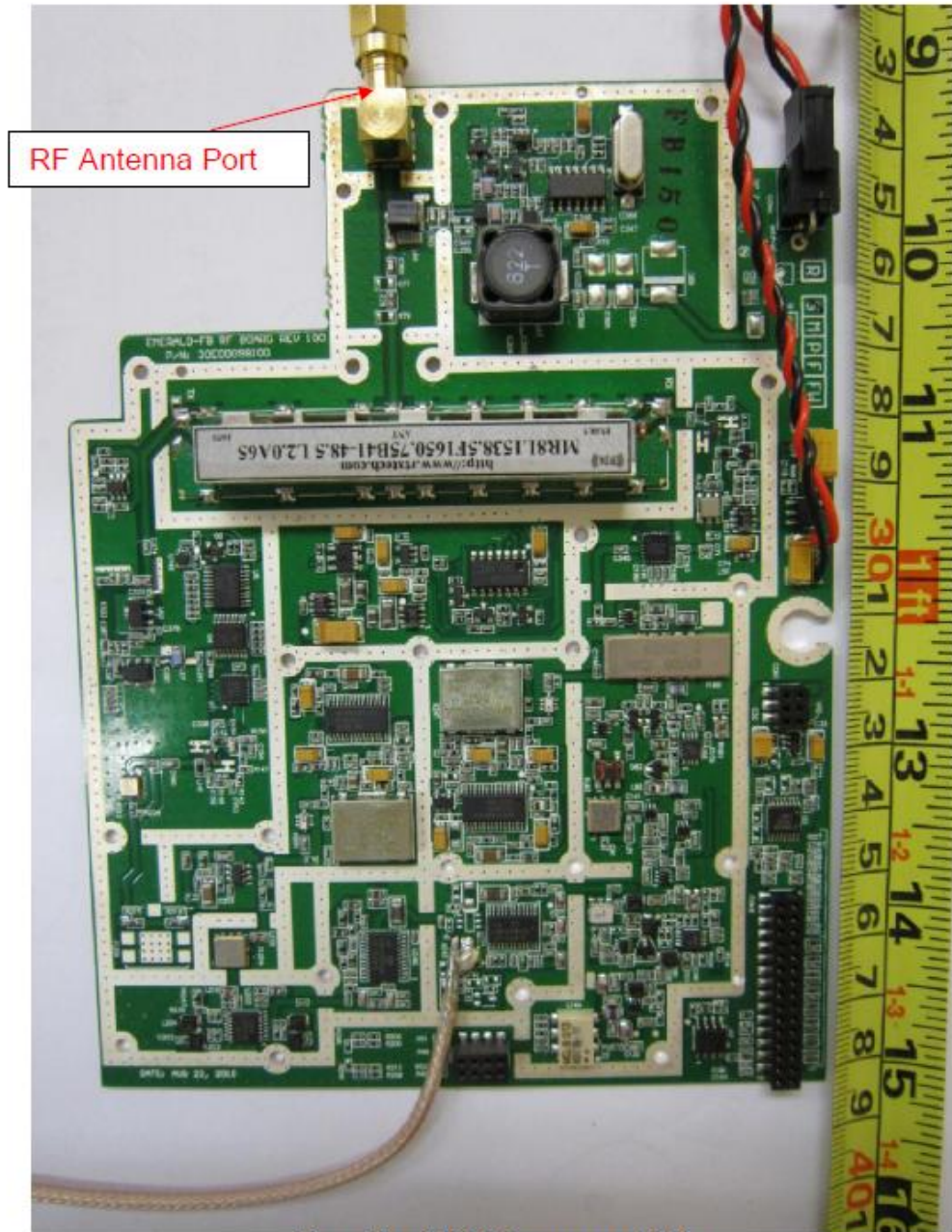
Base Band PCB Component Side
