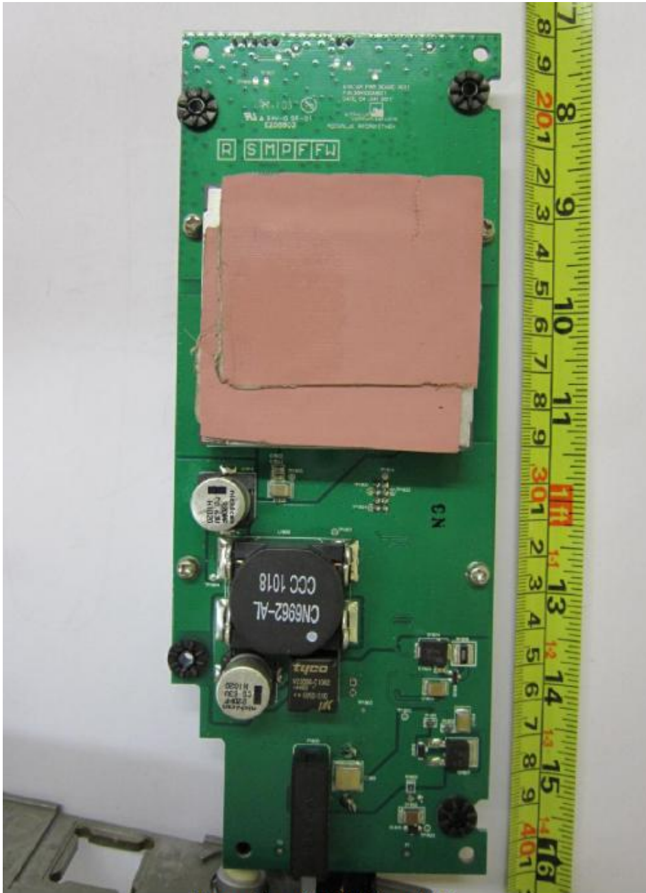
Power Supply PCB Trace Side
