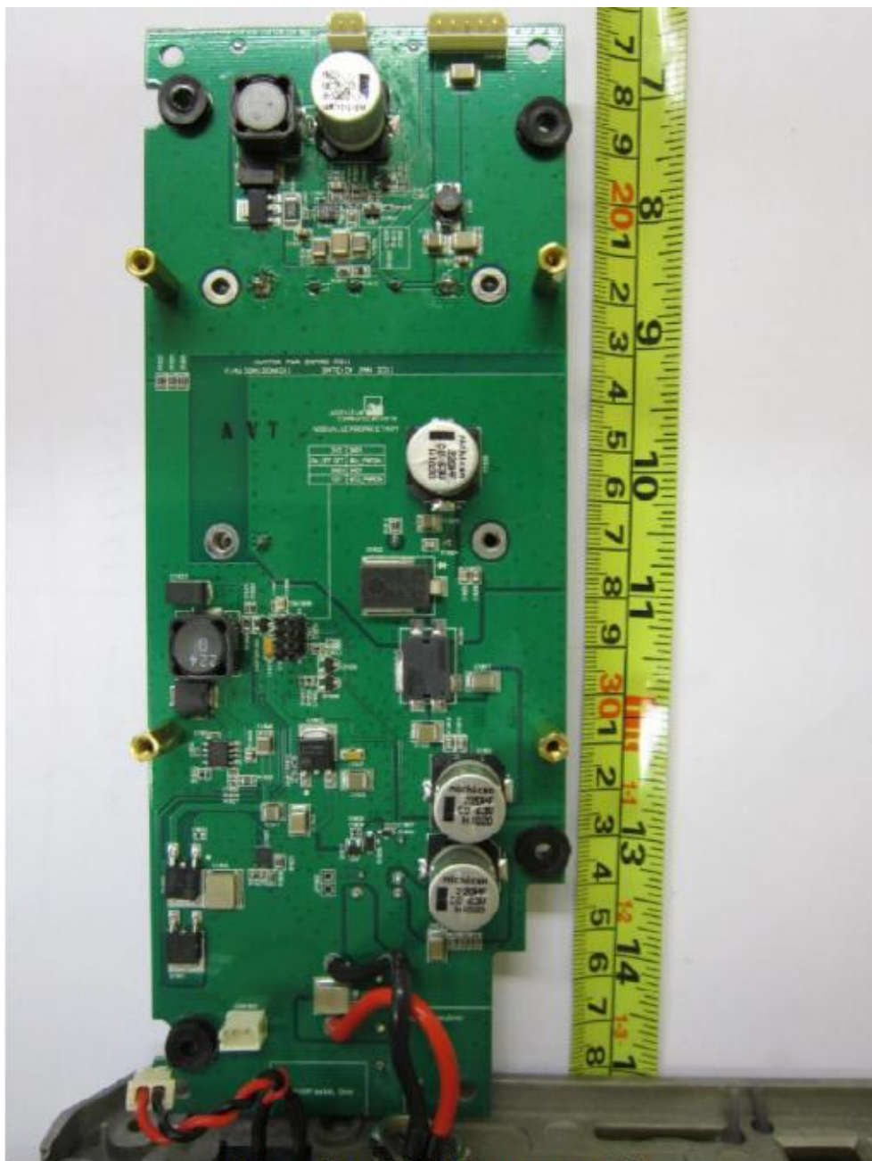
Power Supply PCB Component Side
