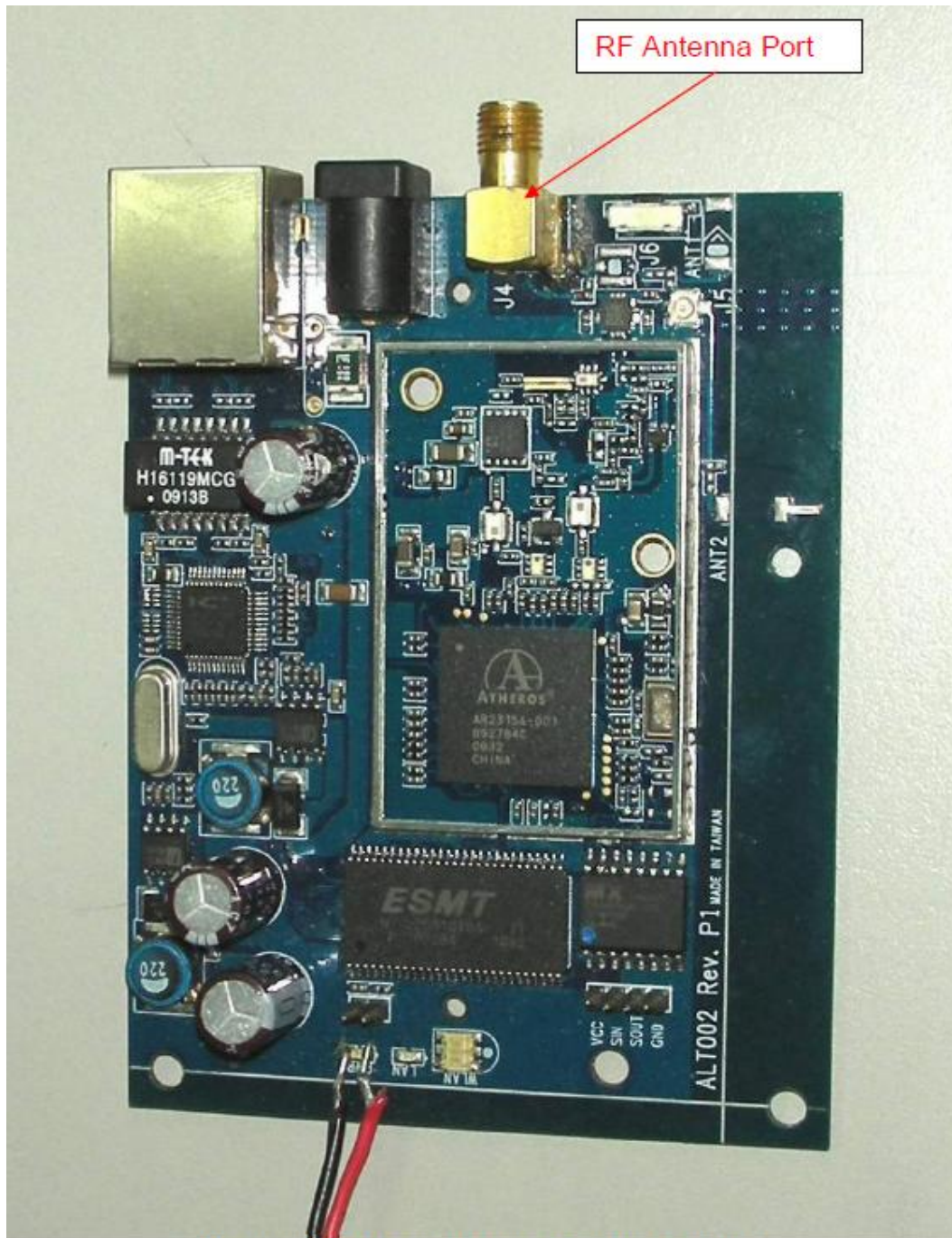
802.11b/g Module Circuit with RF Shield Removed
