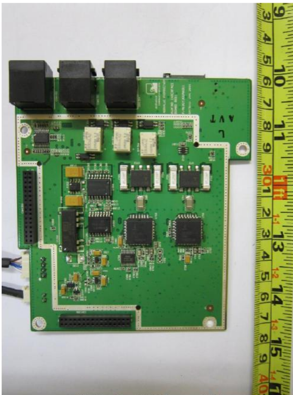
Interface Board PCB Component Side
