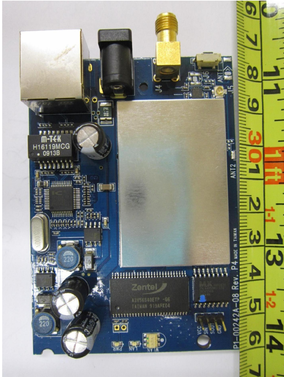
802.11b/g PCB Component Side
