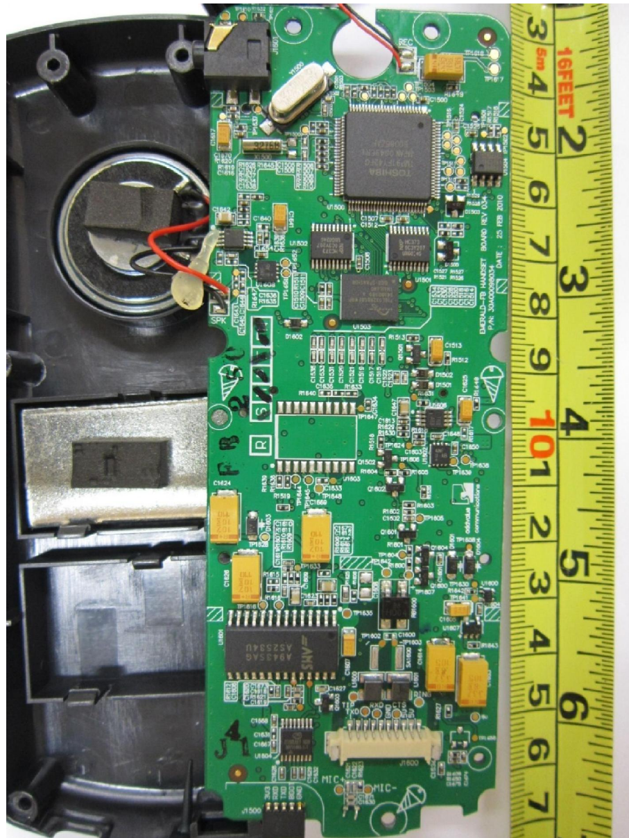
Main-Board Trace View
