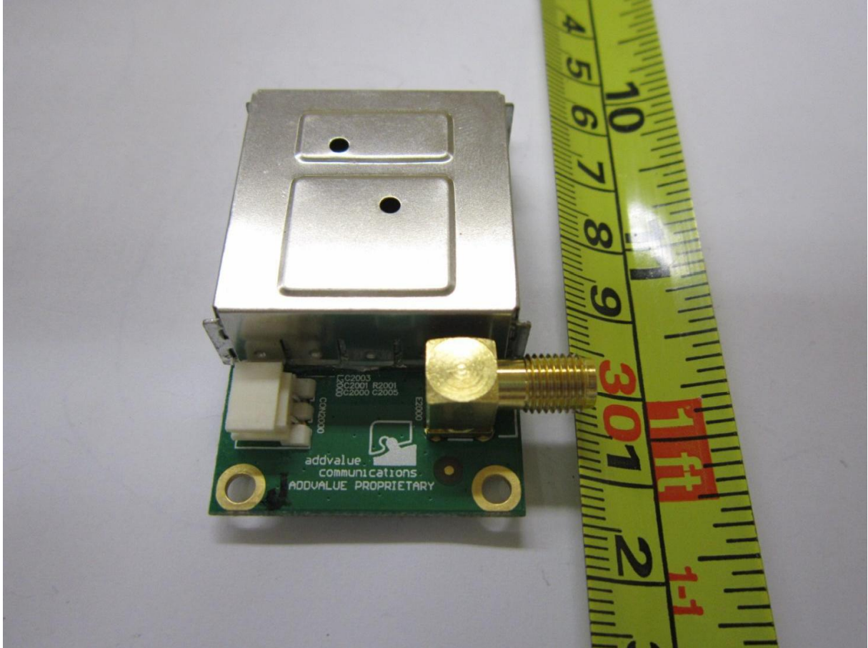
RF Crystal PCB Component Side
