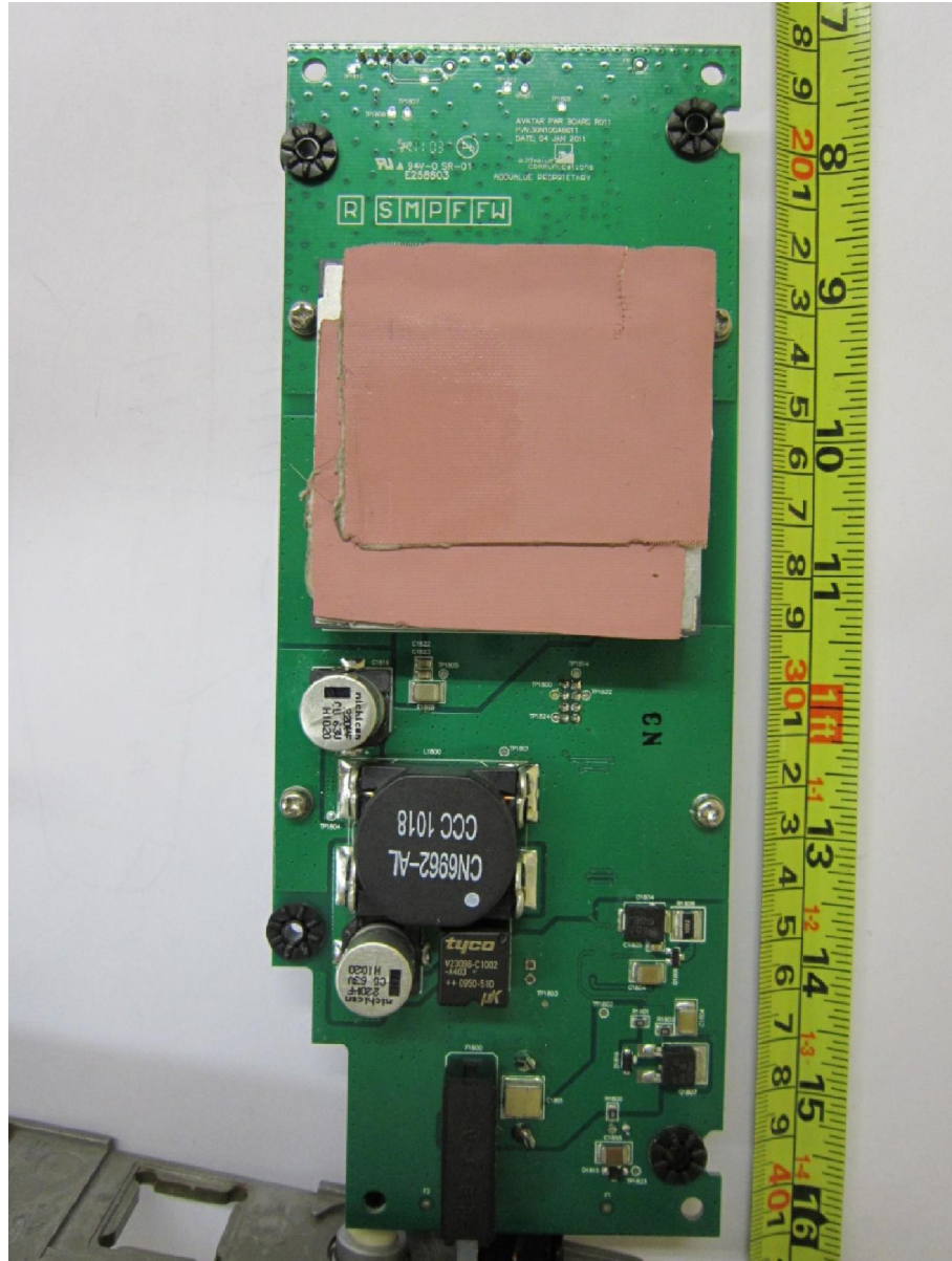
Power Supply PCB Trace Side
