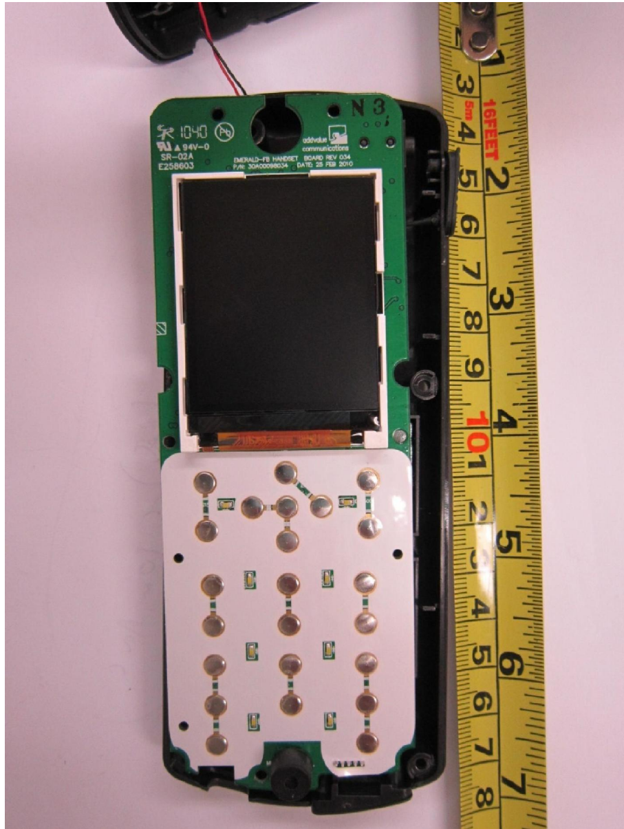
Main-Board Component View
