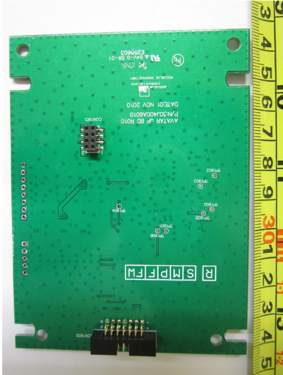
PS-Microprocessor PCB Trace Side
