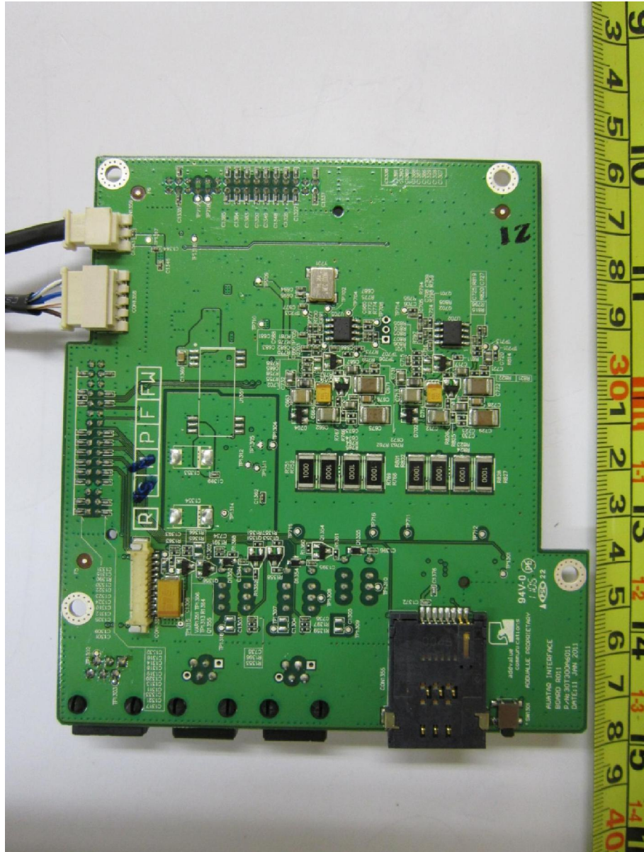
Interface Board PCB Trace Side
