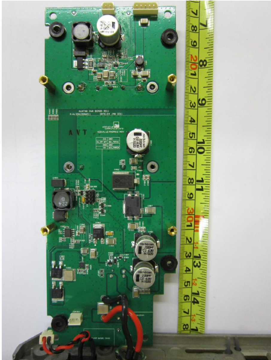
Power Supply PCB Component Side
