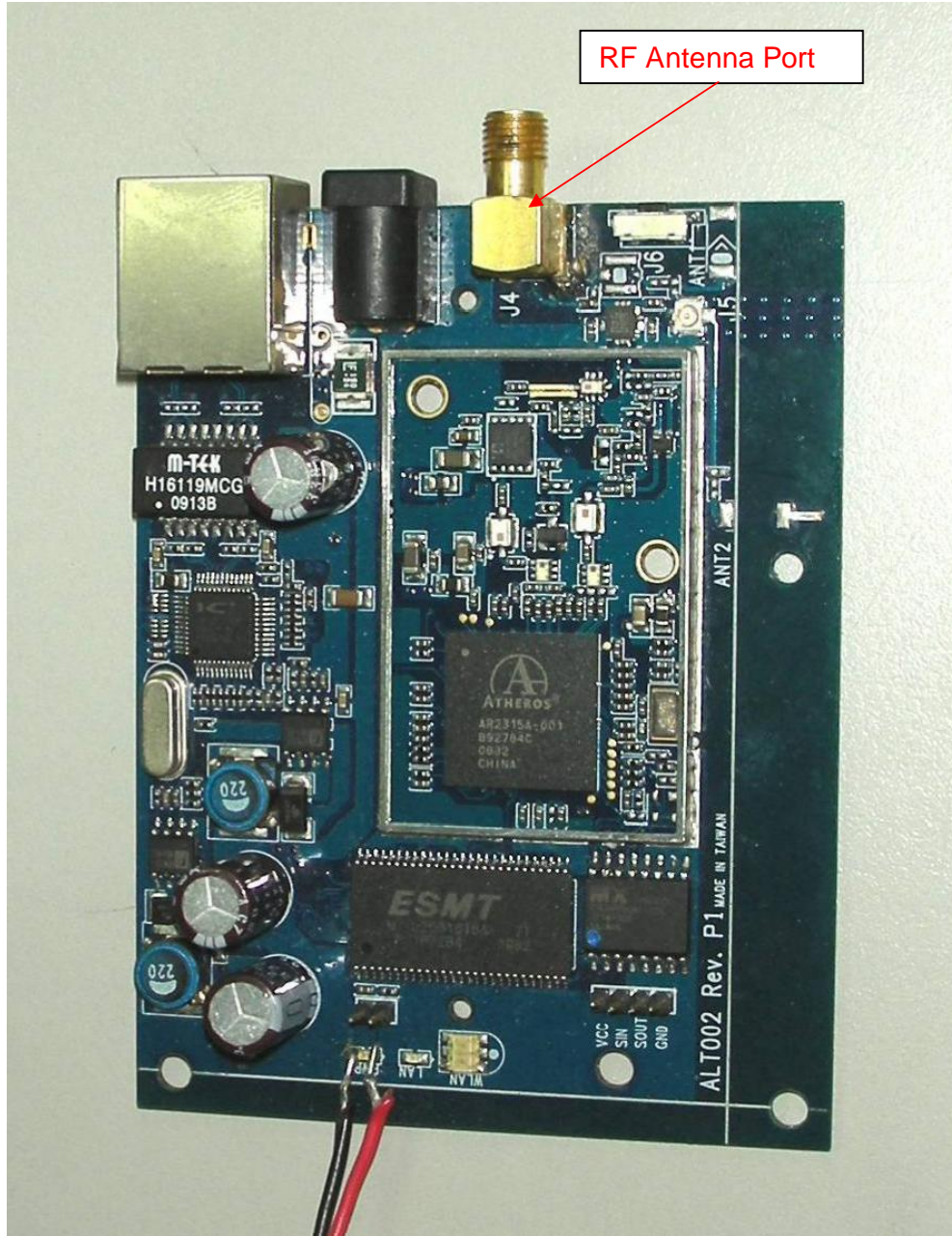
802.11b/g Module Circuit with RF Shield Removed
