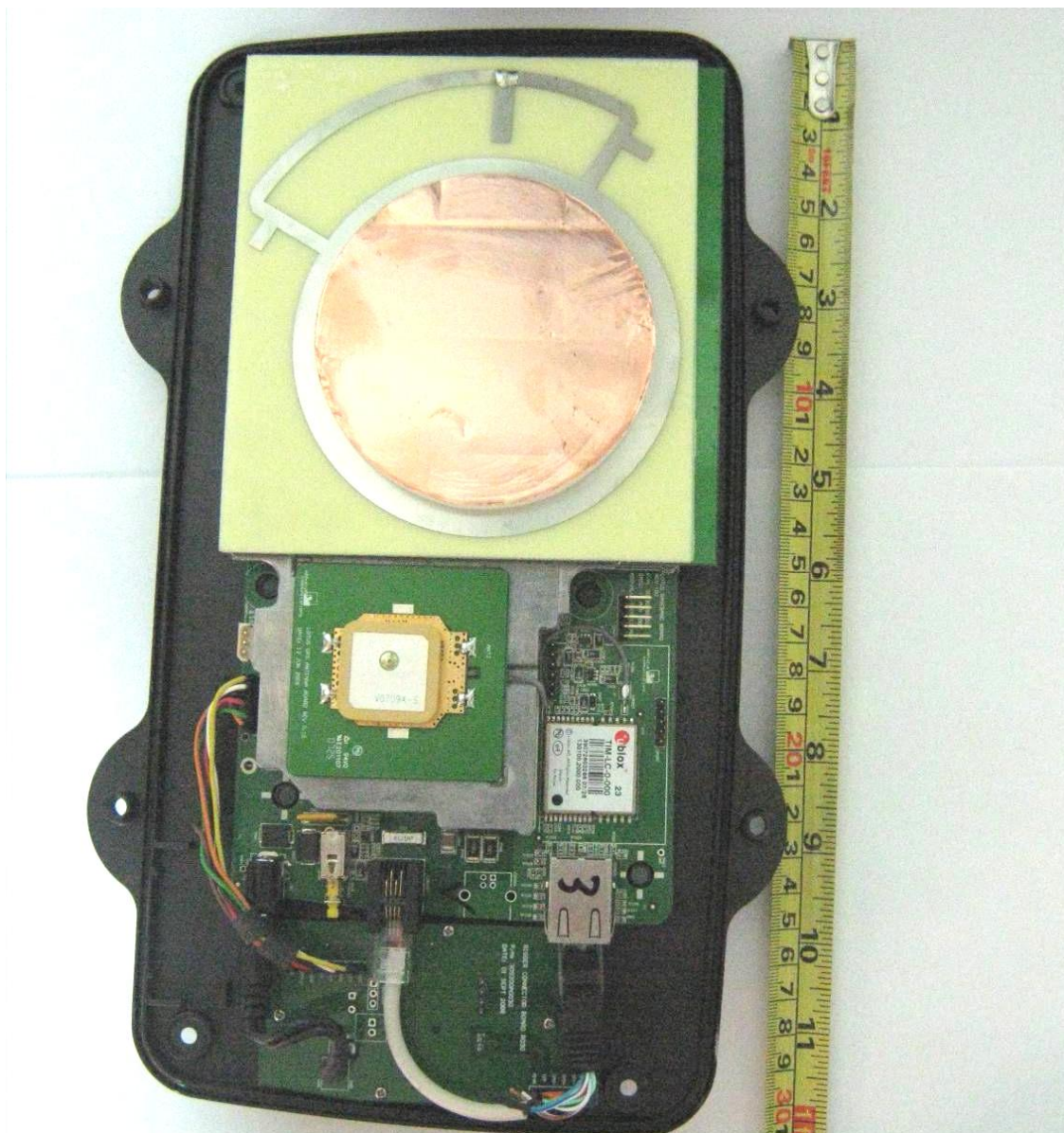
Internal View
