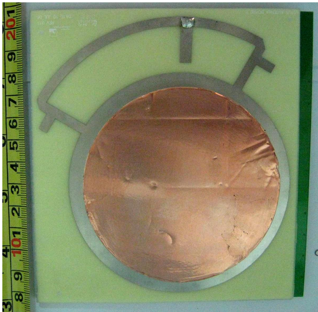
Lotus UT Antenna Board PCB Component Side
