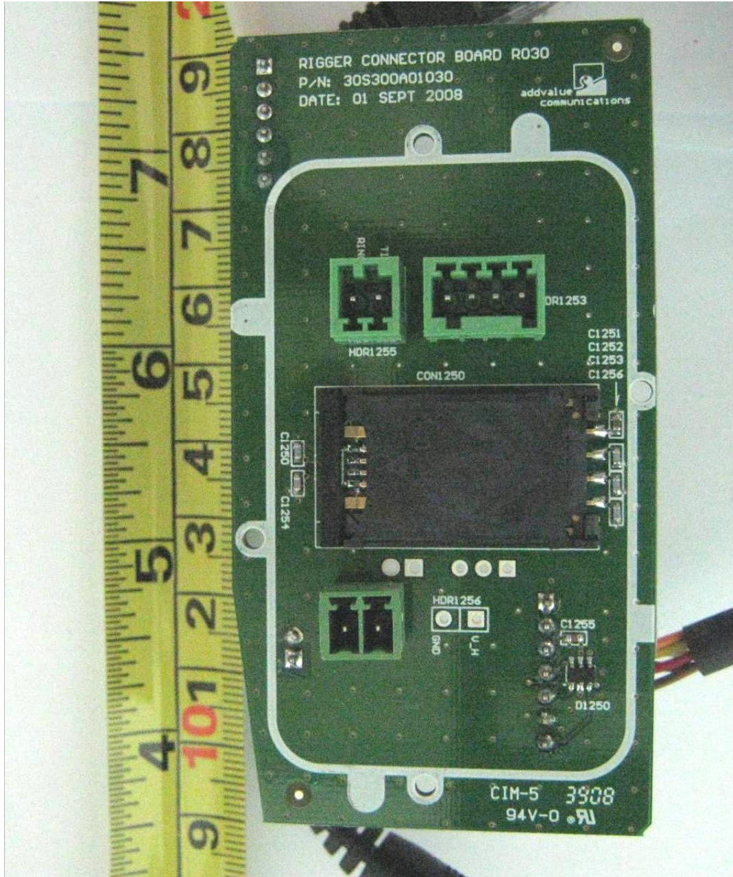
Rigger Connector Board PCB Component Side
